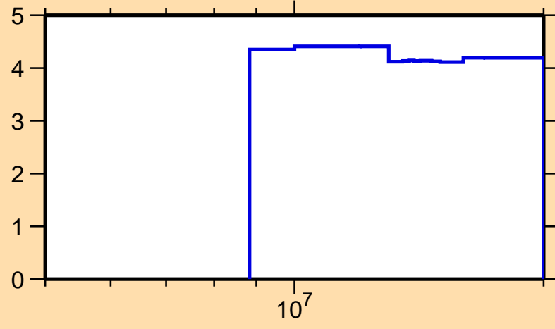
\Delta\sigma/\sigma vs. E for ^{174}\text{W}(n,\text{nonel.})
