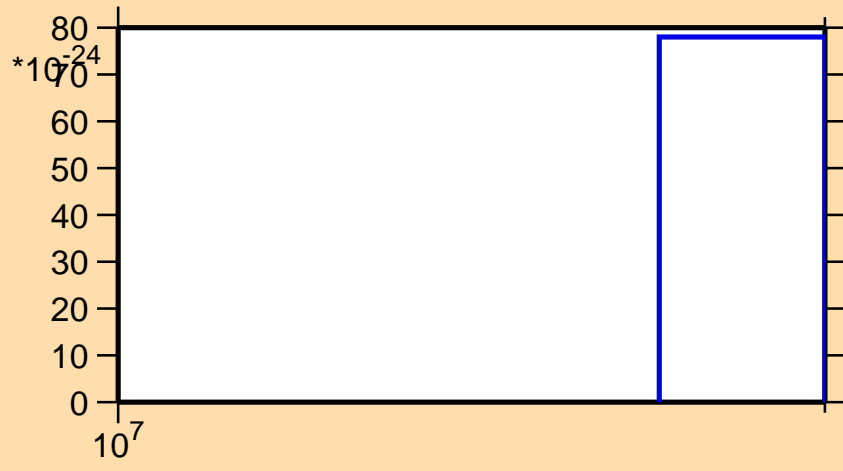
\sigma vs. E for ^{174}\text{W} (mt 11)
