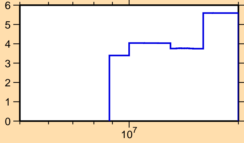
\Delta\sigma/\sigma vs. E for ^{174}\text{W}(n,\text{el.})
