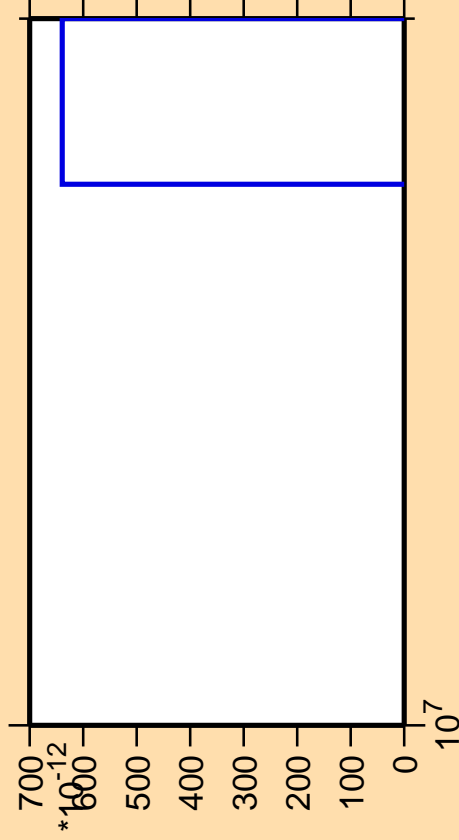
\Delta\sigma/\sigma vs. E for ^{174}\text{W} (mt 11)
