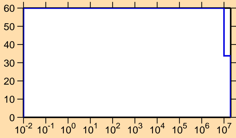
\Delta\sigma/\sigma vs. E for ^{174}\text{W}(n,p)
