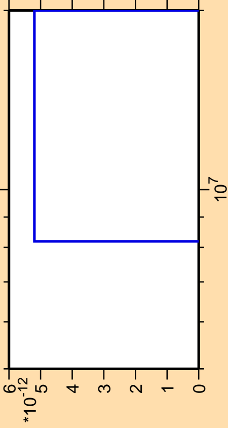
\Delta\sigma/\sigma vs. E for ^{174}\text{W} (mt 11)
