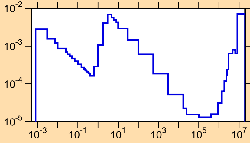
\sigma vs. E for ^{174}\text{W}(n,\alpha)
