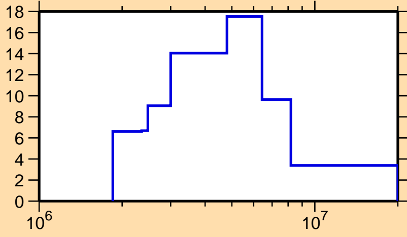
\Delta\sigma/\sigma vs. E for ^{174}\text{W}(n, el.)
