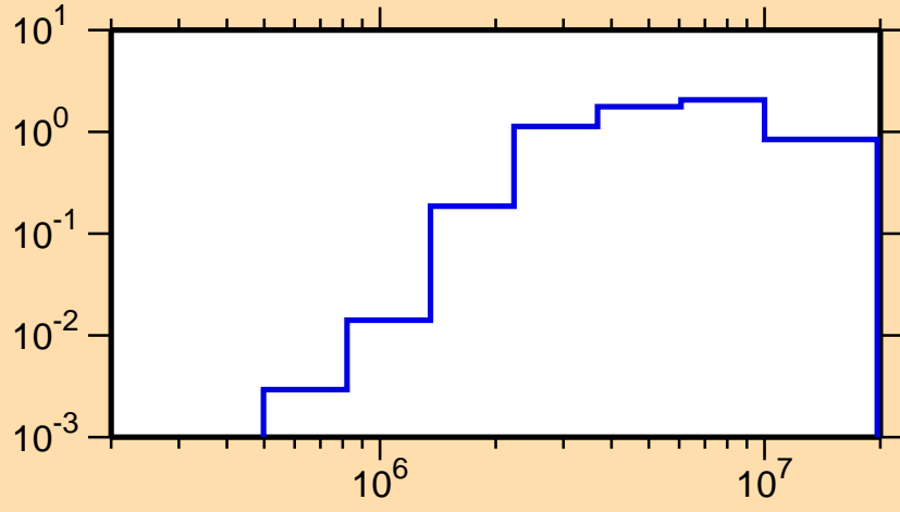
\sigma vs. E for ^{175}\text{W}(n,n\text{cont.})
