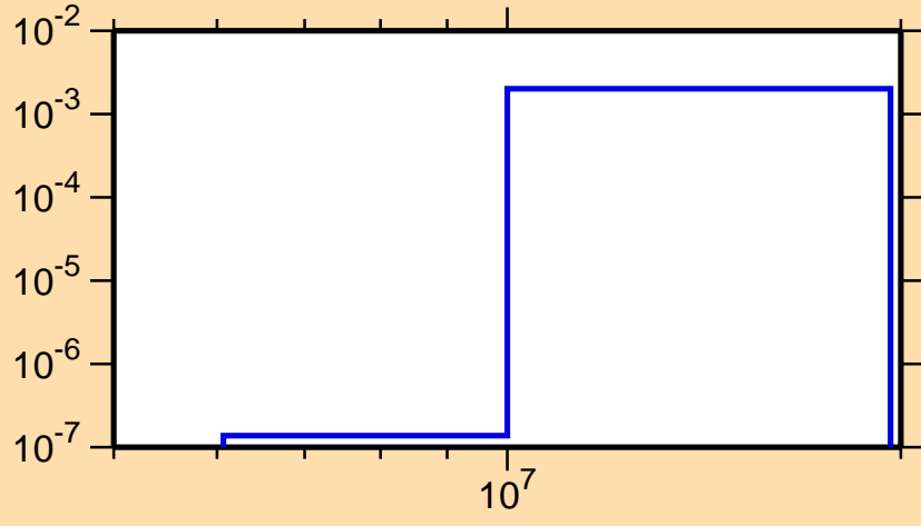
\sigma vs. E for ^{175}\text{W}(n,d)
