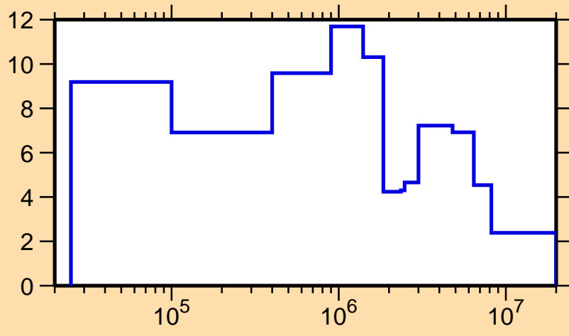
\Delta\sigma/\sigma vs. E for ^{175}\text{W}(n,\text{tot.})
