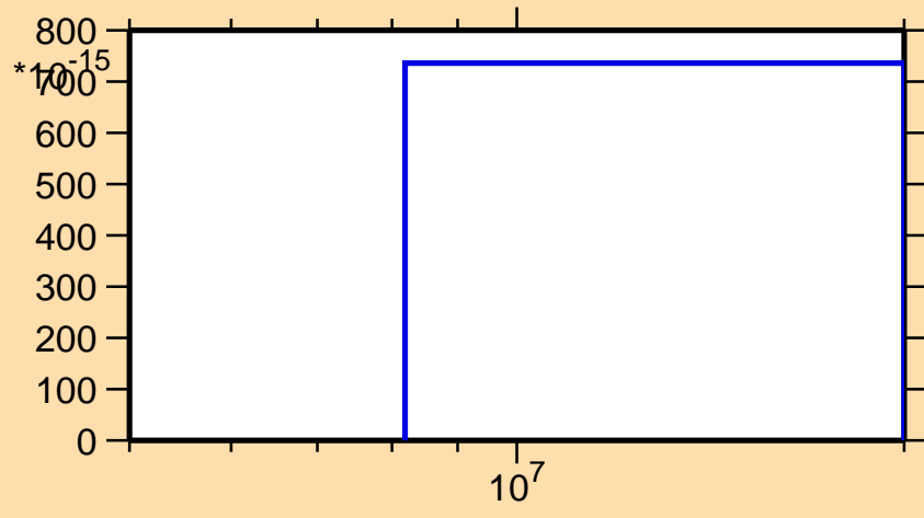
\sigma vs. E for ^{175}\text{W}(\text{mt117})
