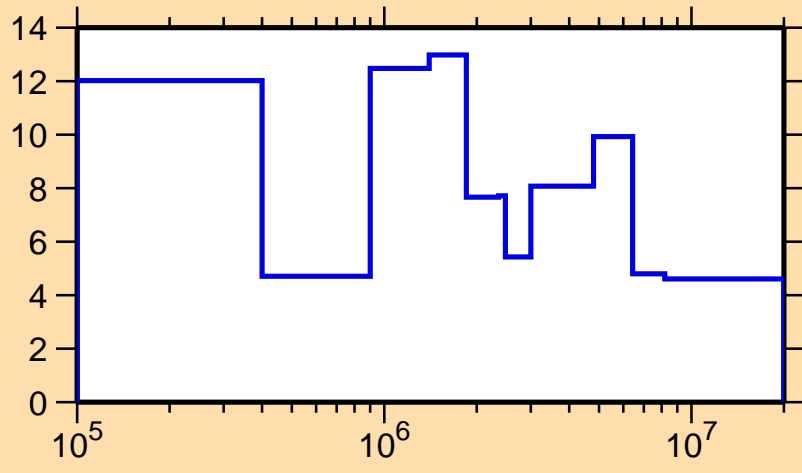
\Delta\sigma/\sigma vs. E for ^{175}\text{W}(n, el.)
