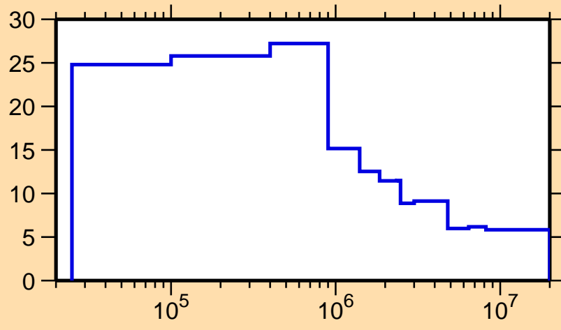
\Delta\sigma/\sigma vs. E for ^{175}\text{W}(n,\text{nonel.})
