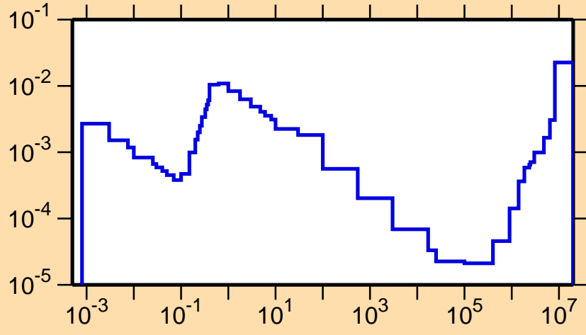
\sigma vs. E for ^{175}\text{W}(n,p)
