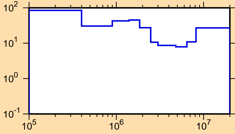
\Delta\sigma/\sigma vs. E for ^{175}\text{W}(n,n\text{cont.})
