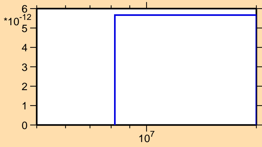
\sigma vs. E for ^{175}\text{W} (mt 45)
