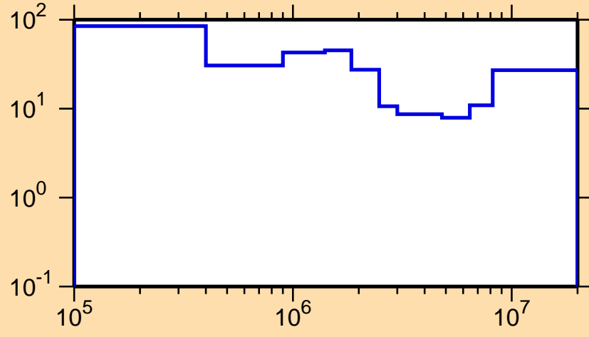
\Delta\sigma/\sigma vs. E for ^{175}\text{W}(n,ncont.)
