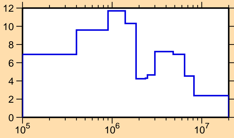
\Delta\sigma/\sigma vs. E for ^{175}\text{W}(n, tot.)
