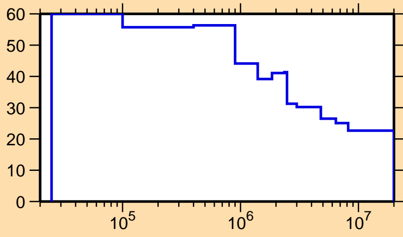
\Delta\sigma/\sigma vs. E for ^{175}\text{W}(n,n_1)
