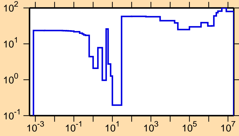
\Delta\sigma/\sigma vs. E for ^{175}\text{W}(n,\gamma)
