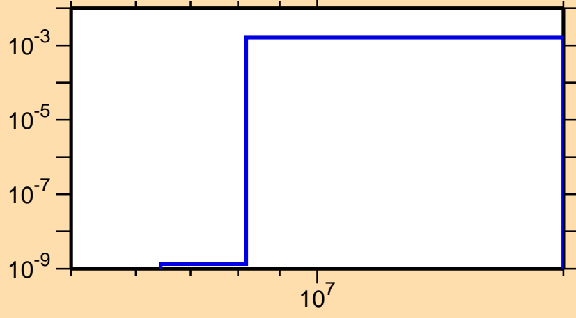
\sigma vs. E for ^{175}\text{W}(n,d)
