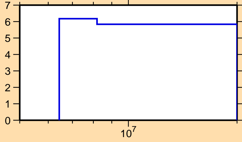
\Delta\sigma/\sigma vs. E for ^{175}\text{W}(n,\text{nonel.})
