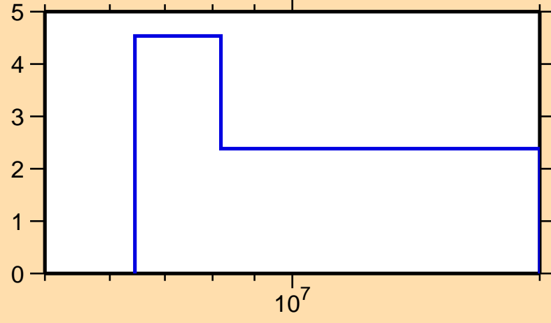
\Delta\sigma/\sigma vs. E for ^{175}\text{W}(n,\text{tot.})
