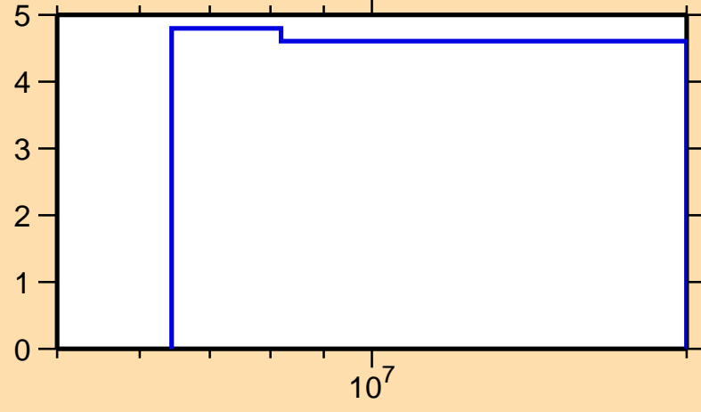
\Delta\sigma/\sigma vs. E for ^{175}\text{W}(n,\text{el.})
