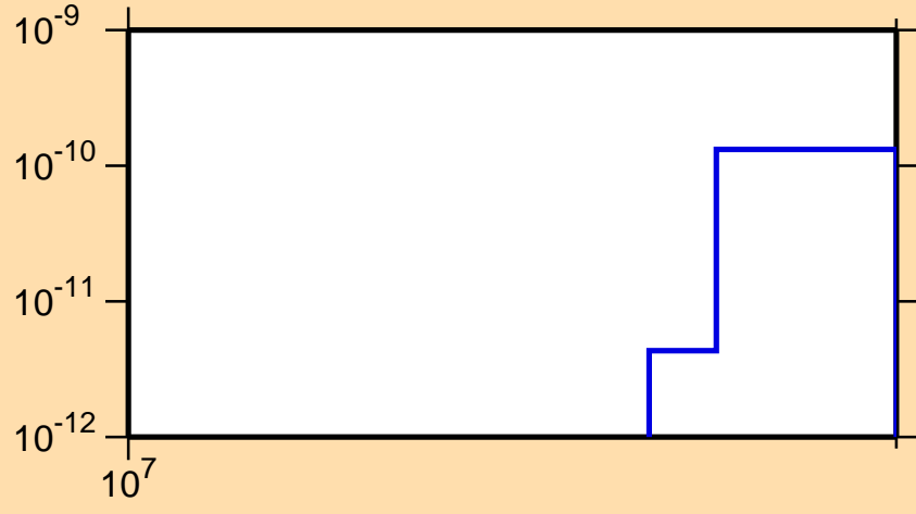
\sigma vs. E for ^{176}\text{W}(n,\text{pd})
