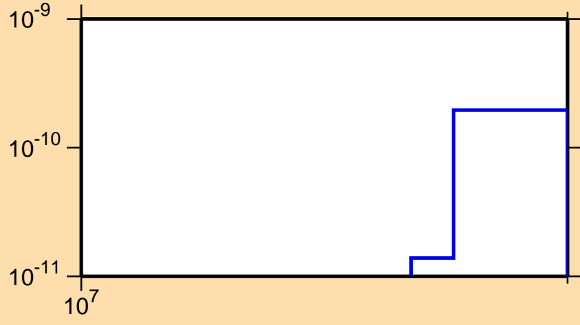
\sigma vs. E for ^{176}\text{W} (mt 45)
