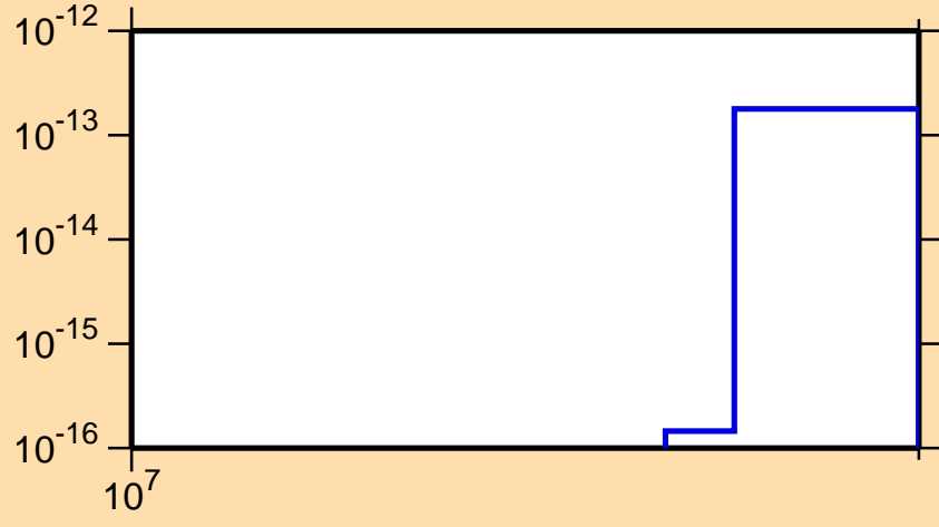
\sigma vs. E for ^{176}\text{W} (mt 34)
