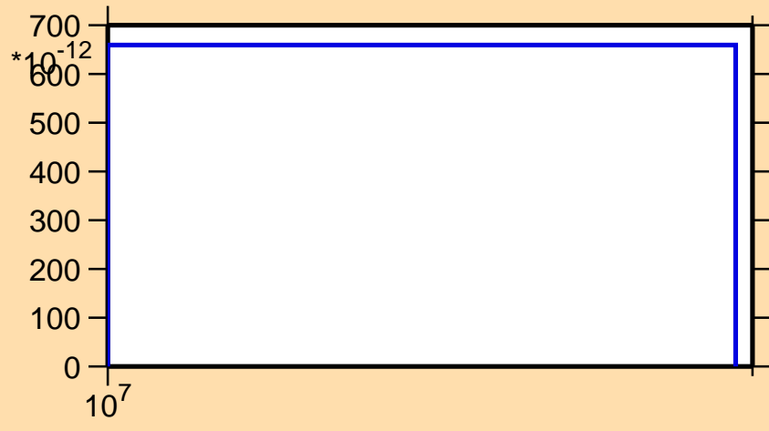
\sigma vs. E for ^{176}\text{W}(n,\text{nd})
