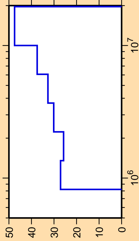
\Delta\sigma/\sigma vs. E for ^{176}\text{W}(n,n_4)
