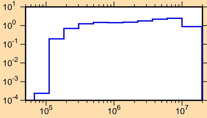
\sigma vs. E for ^{176}\text{W}(n,\text{inel.})
