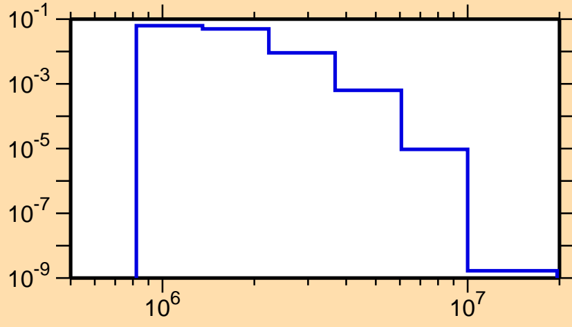
\sigma vs. E for ^{176}\text{W}(n,n_4)
