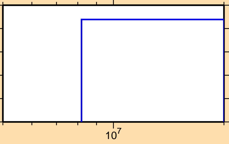
\sigma vs. E for ^{176}\text{W}(n,2n\alpha)
