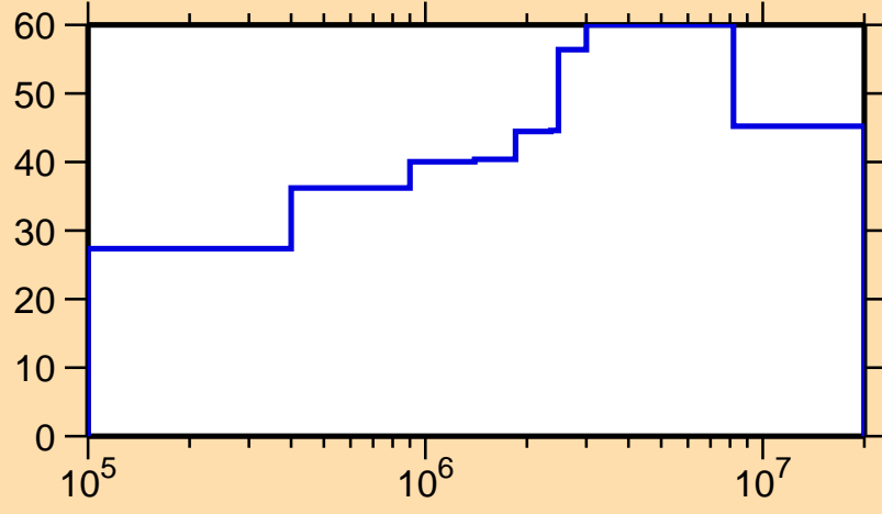
\Delta\sigma/\sigma vs. E for ^{176}\text{W}(n,\gamma)
