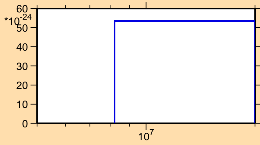
\sigma vs. E for ^{176}\text{W} (mt 11)
