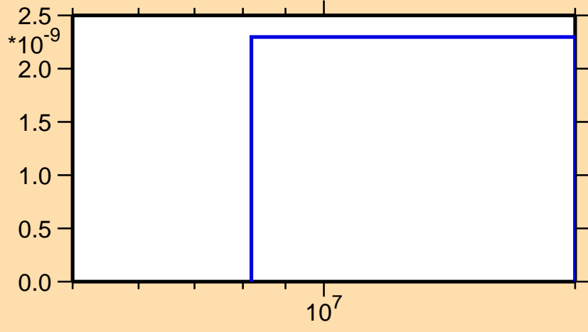
\sigma vs. E for ^{176}\text{W}(n,2np)
