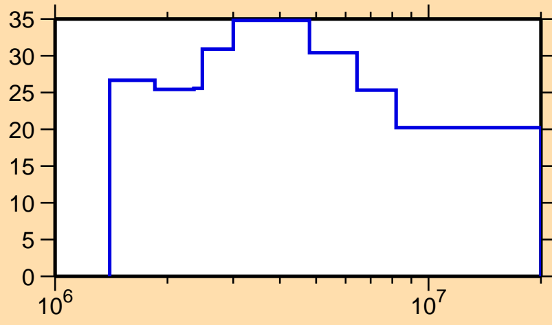
\Delta\sigma/\sigma vs. E for ^{176}\text{W}(n,n_1)
