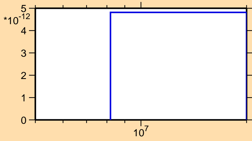
\sigma vs. E for ^{176}\text{W}(n,nt)
