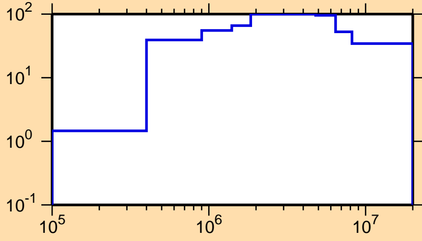
\Delta\sigma/\sigma vs. E for ^{176}\text{W}(n,p)
