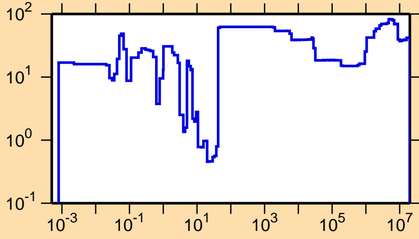
\Delta\sigma/\sigma vs. E for ^{177}\text{W}(n,\gamma)
