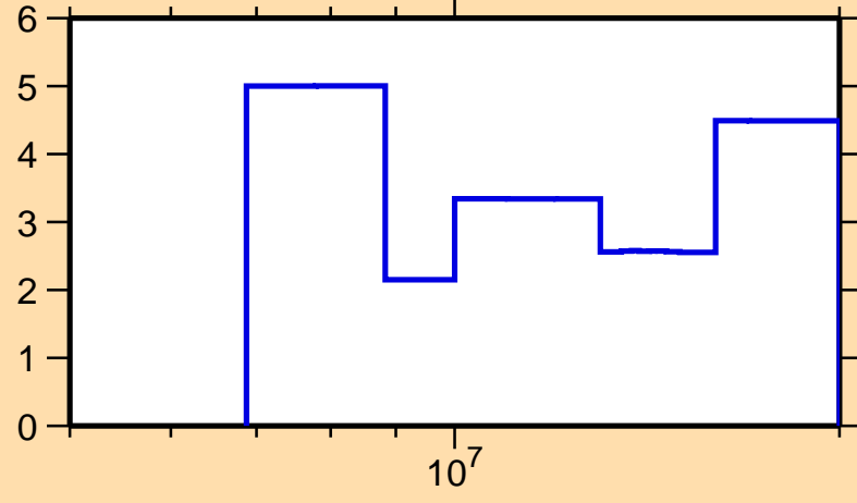
\Delta\sigma/\sigma vs. E for ^{177}\text{W}(n,\text{el.})
