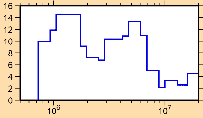
\Delta\sigma/\sigma vs. E for ^{177}\text{W}(n, el.)
