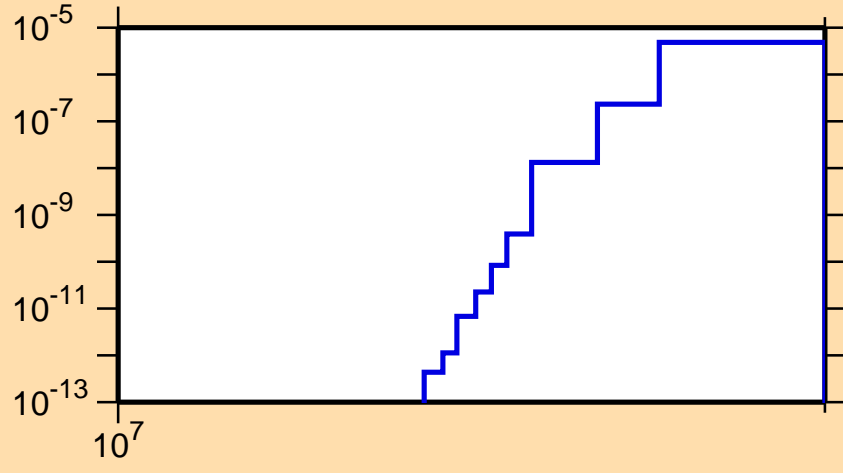
\sigma vs. E for ^{177}\text{W}(n,\text{nd})
