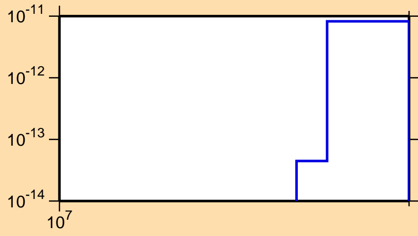
\sigma vs. E for ^{177}\text{W}(n,\text{pt})
