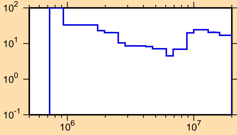
\Delta\sigma/\sigma vs. E for ^{177}\text{W}(n,n\text{cont.})
