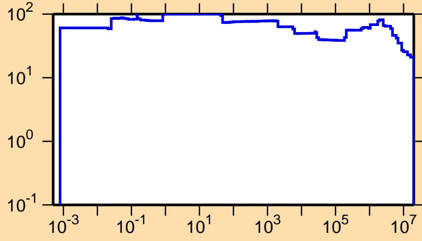
\Delta\sigma/\sigma vs. E for ^{177}\text{W}(n,p)
