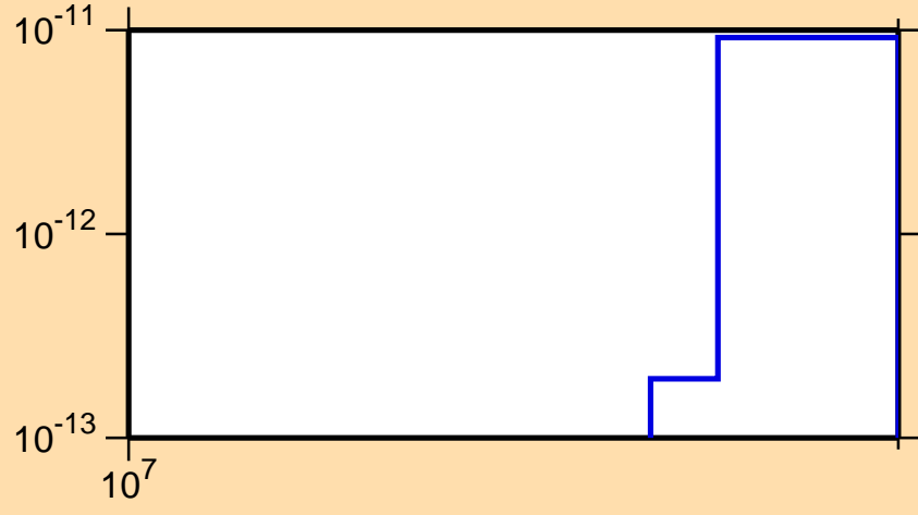
\sigma vs. E for ^{177}\text{W}(n,\text{pd})
