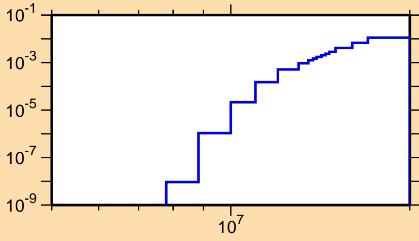
\sigma vs. E for ^{177}\text{W}(n,np)
