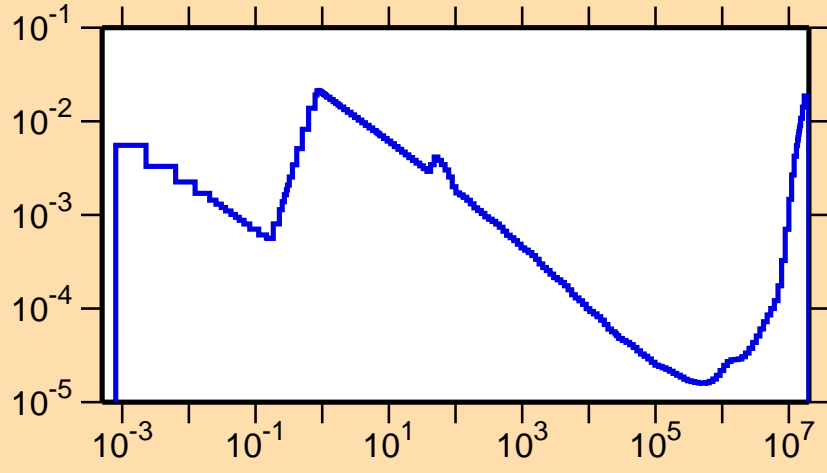
\sigma vs. E for ^{177}\text{W}(n,\alpha)
