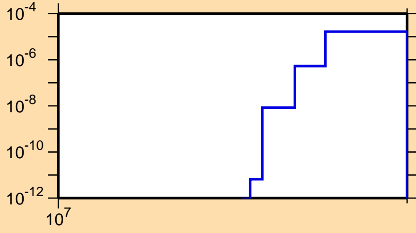
\sigma vs. E for ^{177}\text{W}(n,2np)
