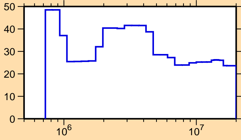
\Delta\sigma/\sigma vs. E for ^{177}\text{W}(n,n_1)
