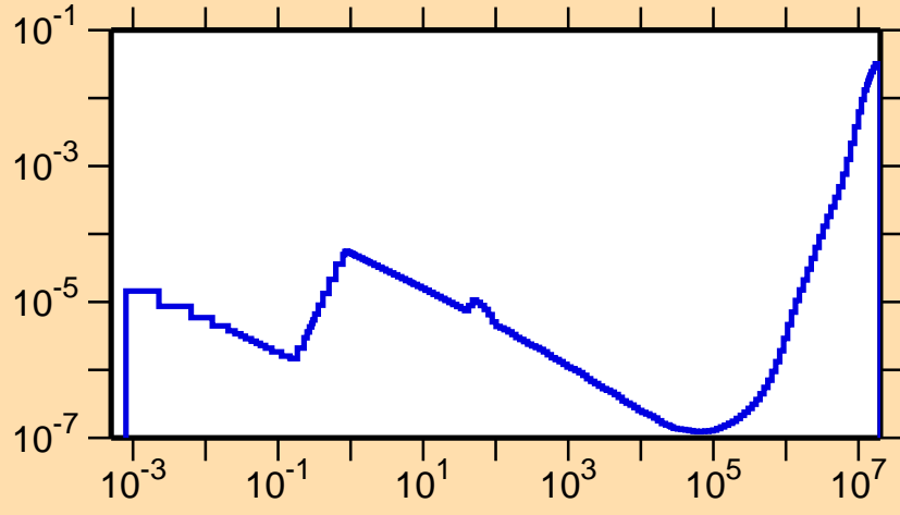
\sigma vs. E for ^{177}\text{W}(n,p)
