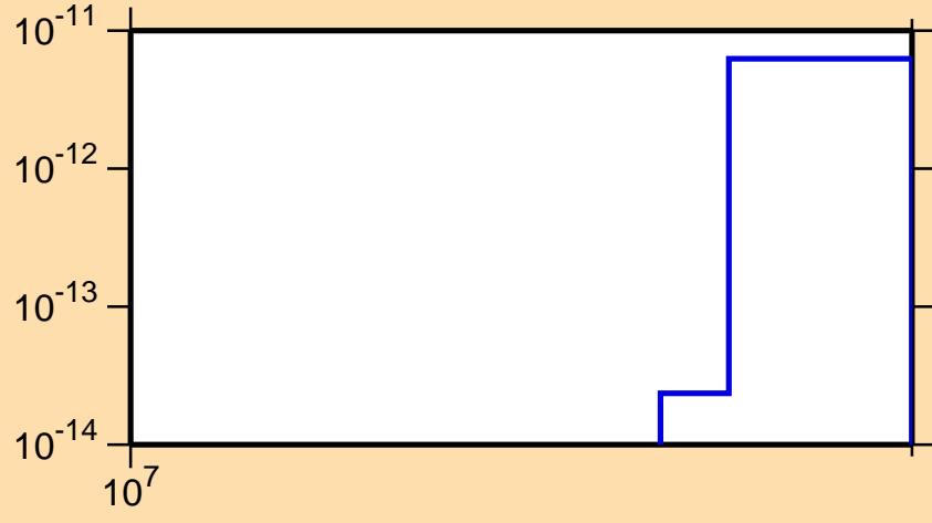
\sigma vs. E for ^{177}\text{W} (mt 34)
