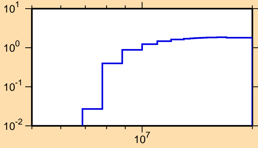
\sigma vs. E for ^{177}\text{W}(n,2n)
