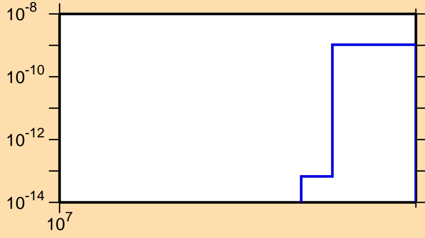
\sigma vs. E for ^{177}\text{W}(n,nt)
