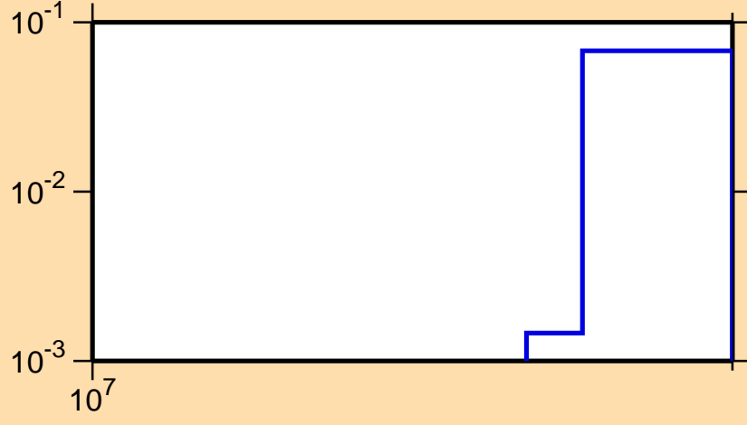
\sigma vs. E for ^{177}\text{W}(n,3n)
