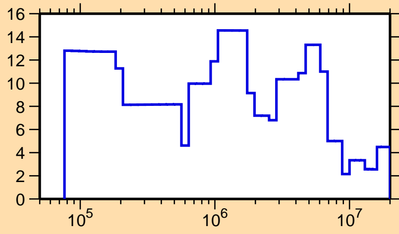
\Delta\sigma/\sigma vs. E for ^{177}\text{W}(n,\text{el.})
