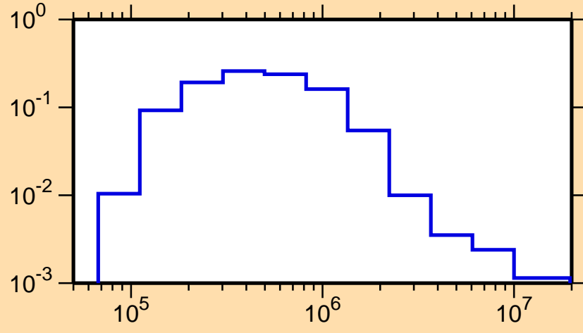
\sigma vs. E for ^{177}\text{W}(n,n_2)
