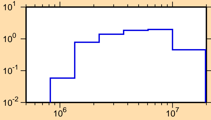
\sigma vs. E for ^{177}\text{W}(n,n\text{cont.})
