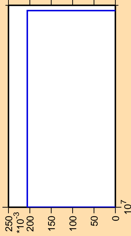
\Delta\sigma/\sigma vs. E for ^{177}\text{W} (mt 34)
