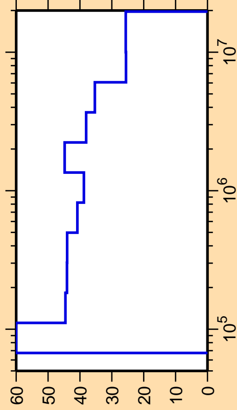
\Delta\sigma/\sigma vs. E for ^{177}\text{W}(n,n_2)
