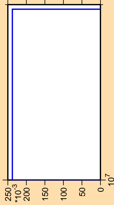
\Delta\sigma/\sigma vs. E for ^{177}\text{W}(n,\text{pt})
