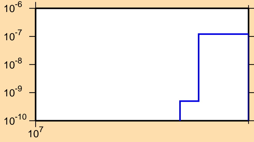
\sigma vs. E for ^{178}\text{W}(n,\text{nd})
