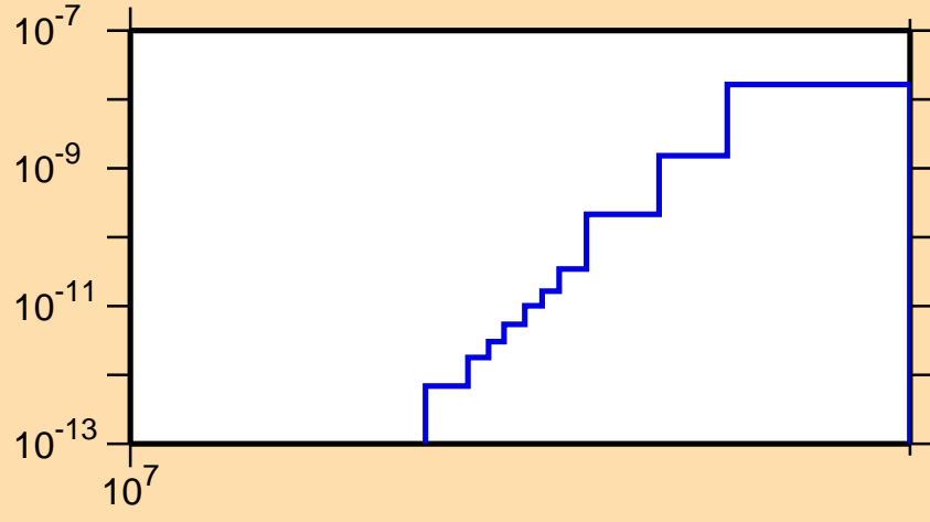
\sigma vs. E for ^{178}\text{W}(n,\text{He3})
