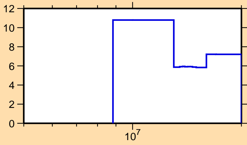
\Delta\sigma/\sigma vs. E for ^{178}\text{W}(n,2n)
