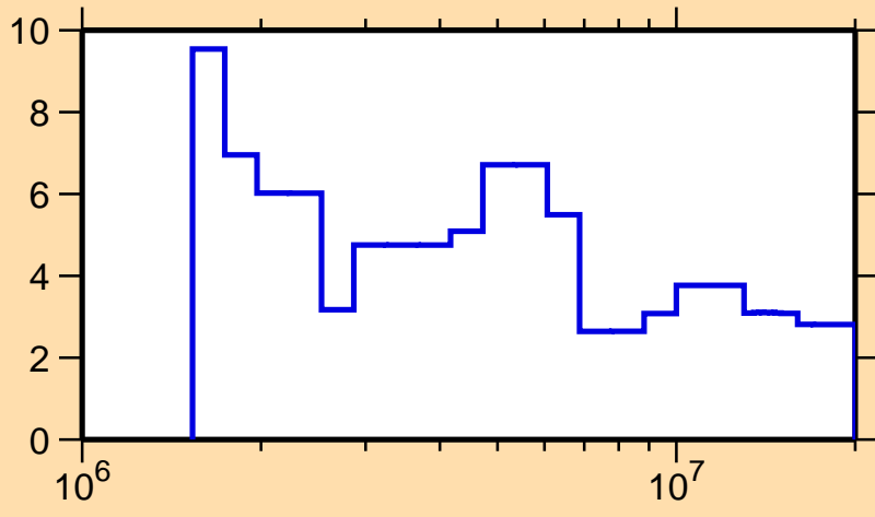
\Delta\sigma/\sigma vs. E for ^{178}\text{W}(n, el.)
