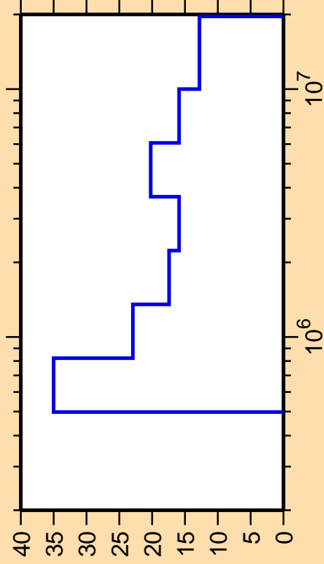
\Delta\sigma/\sigma vs. E for ^{178}\text{W}(n,n_3)
