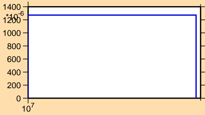
\sigma vs. E for ^{178}\text{W}(n,3n)
