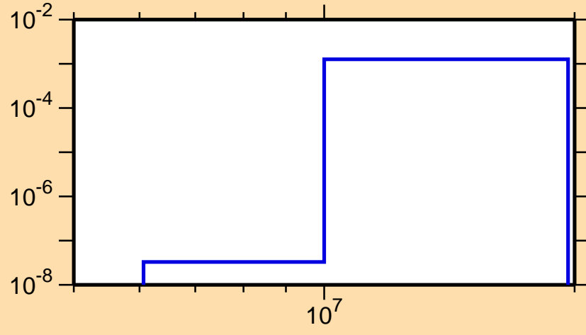
\sigma vs. E for ^{178}\text{W}(n,np)
