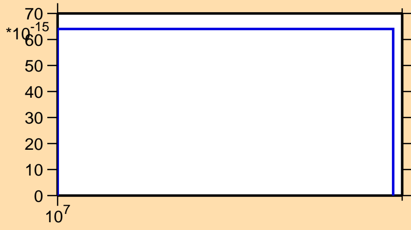
\sigma vs. E for ^{178}\text{W}(\text{mt117})
