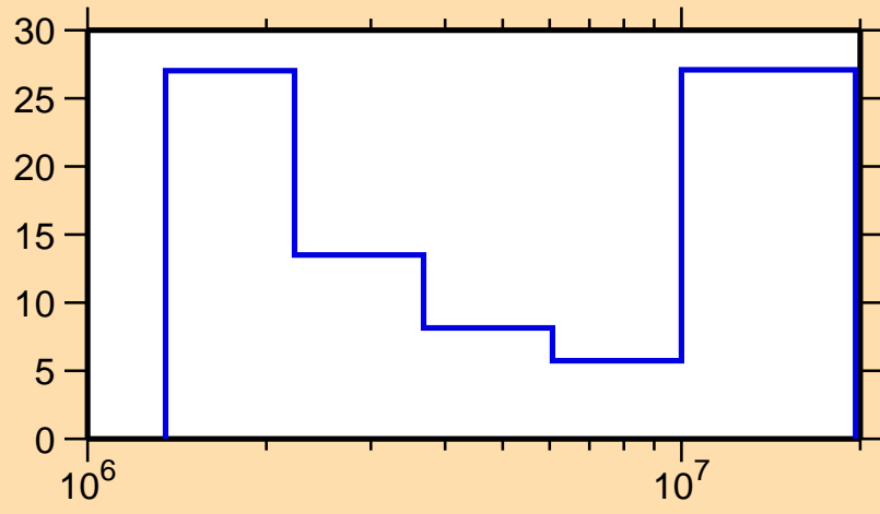
\Delta\sigma/\sigma vs. E for ^{178}\text{W}(n,n\text{cont.})
