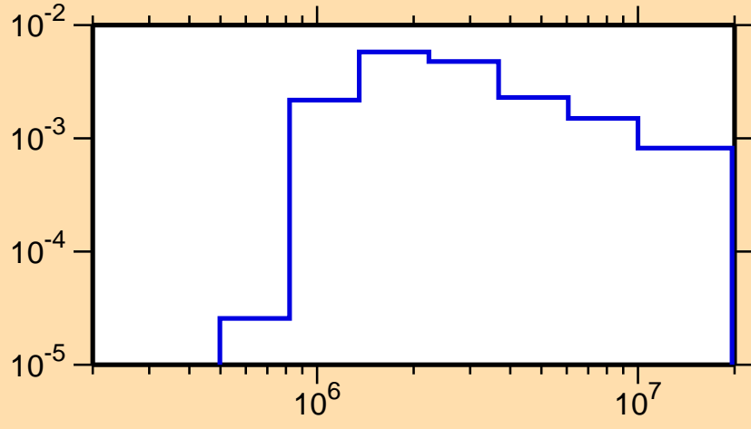
\sigma vs. E for ^{178}\text{W}(n,n_3)
