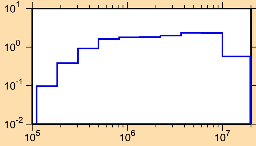
\sigma vs. E for ^{179}\text{W}(n,\text{inel.})
