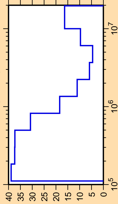
\Delta\sigma/\sigma vs. E for ^{179}\text{W}(n,\text{inel.})
