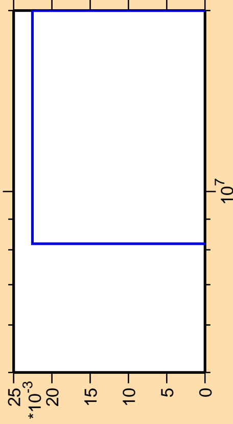
\Delta\sigma/\sigma vs. E for ^{179}\text{W} (mt 45)
