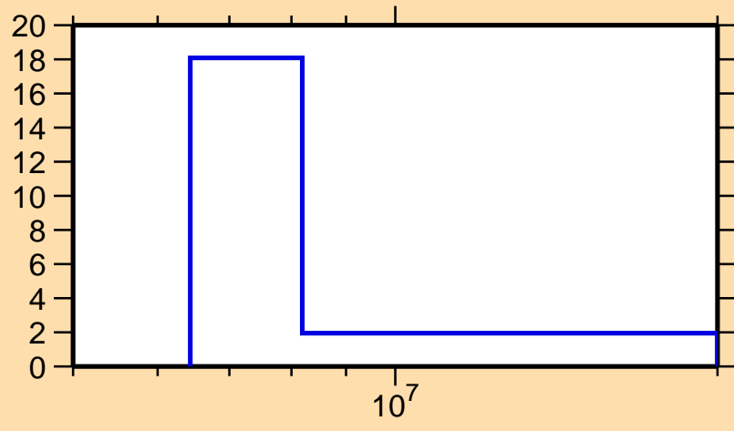
\Delta\sigma/\sigma vs. E for ^{179}\text{W}(n,2n)
