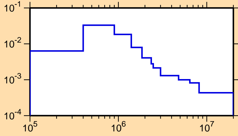
\sigma vs. E for ^{179}\text{W}(n,n_2)
