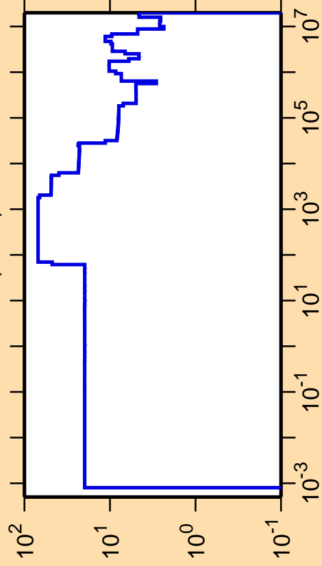
\Delta\sigma/\sigma vs. E for ^{179}\text{W}(n,\text{el.})
