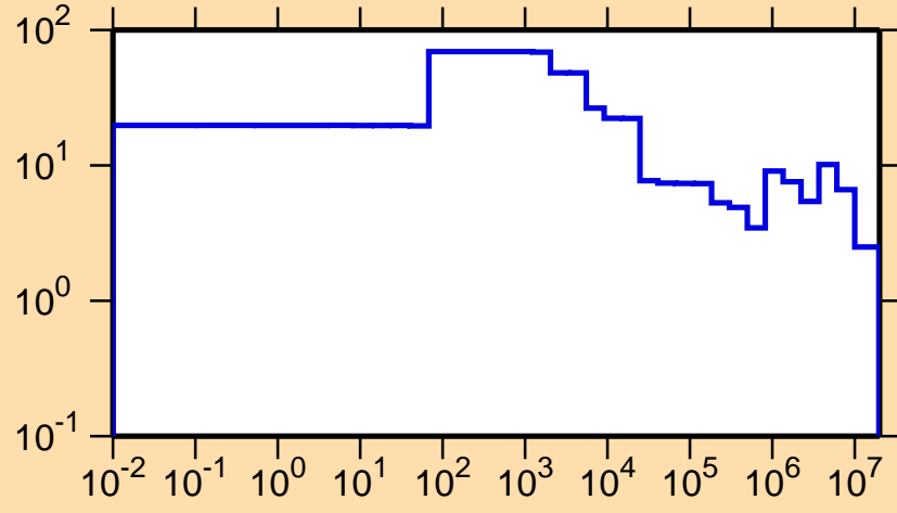
\Delta\sigma/\sigma vs. E for ^{179}\text{W}(n,el.)
