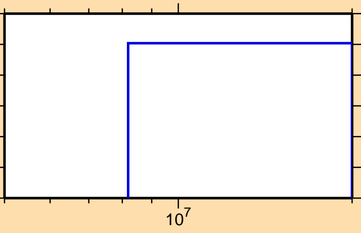
\sigma vs. E for ^{179}\text{W}(n,2np)
