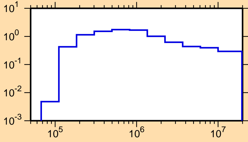
\sigma vs. E for ^{180}\text{W}(n,n_1)
