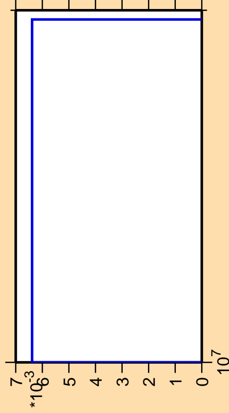
\Delta\sigma/\sigma vs. E for ^{180}\text{W} (mt 45)
