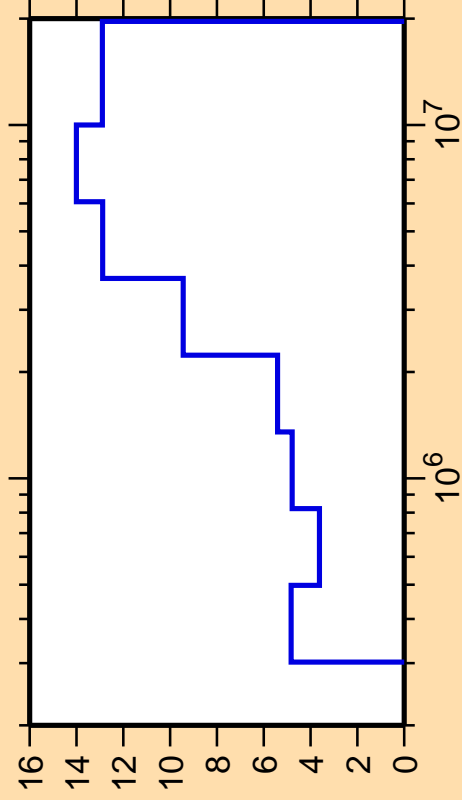
\Delta\sigma/\sigma vs. E for ^{180}\text{W}(n,n_2)
