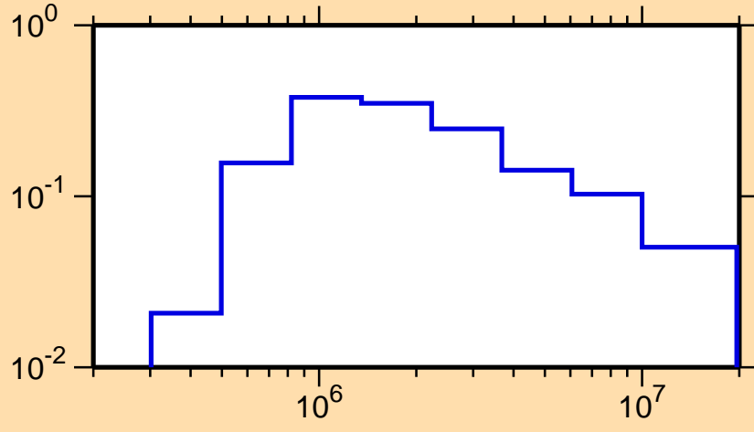
\sigma vs. E for ^{180}\text{W}(n,n_2)
