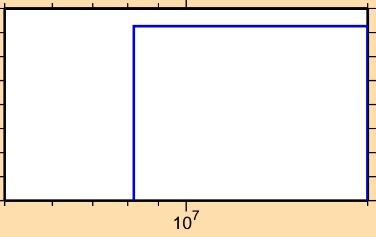
\sigma vs. E for ^{180}\text{W}(n,2n\alpha)
