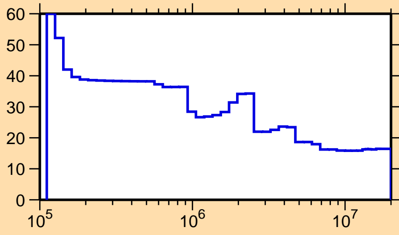
\Delta\sigma/\sigma vs. E for ^{181}\text{W}(n,n_1)
