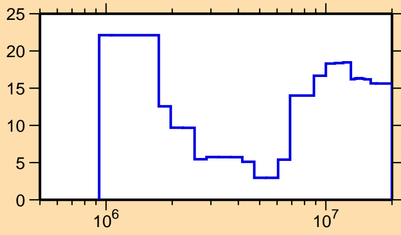
\Delta\sigma/\sigma vs. E for ^{181}\text{W}(n,ncont.)
