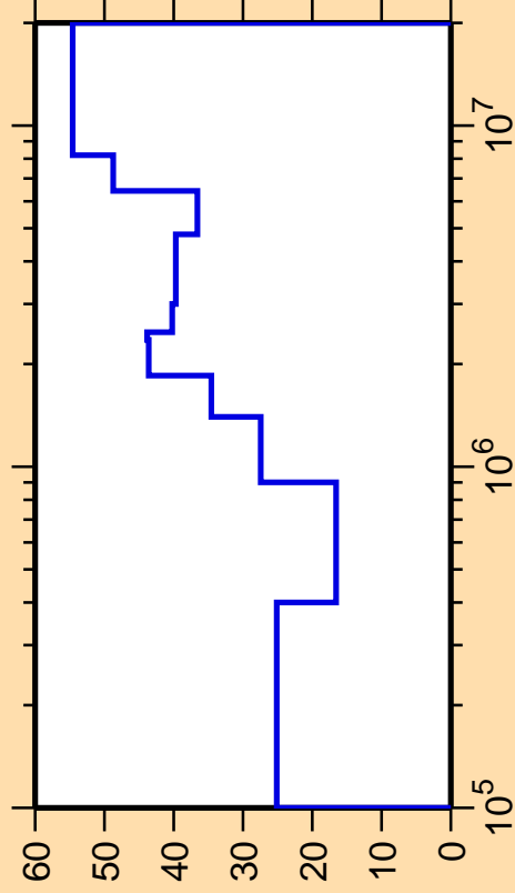
\Delta\sigma/\sigma vs. E for ^{181}\text{W}(n,n_4)
