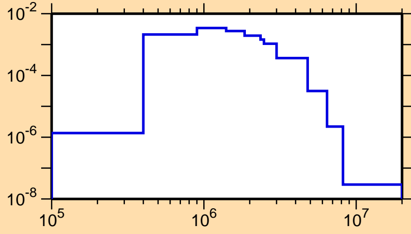
\sigma vs. E for ^{181}\text{W}(n,n_4)
