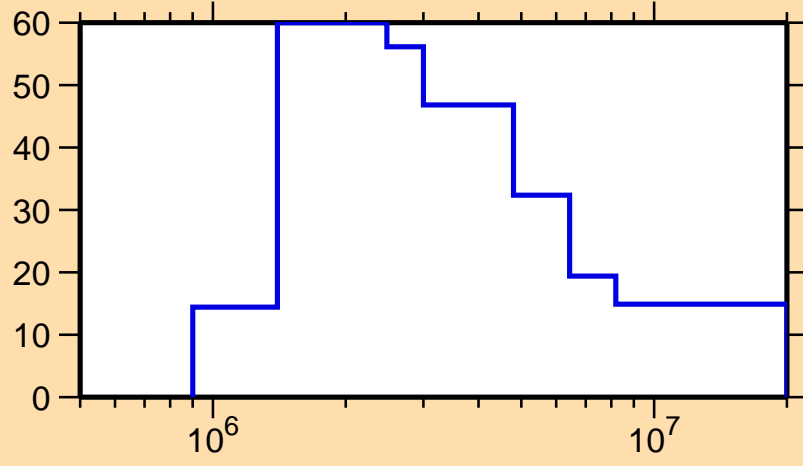
\Delta\sigma/\sigma vs. E for ^{181}\text{W}(n,p)
