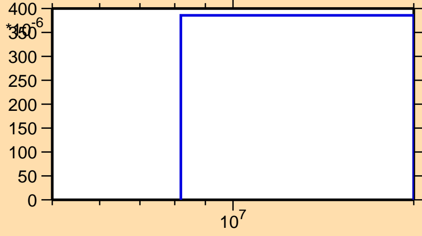
\sigma vs. E for ^{181}\text{W}(n,np)
