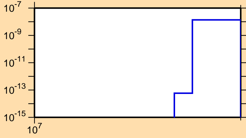
\sigma vs. E for ^{182}\text{W}(n,2np)
