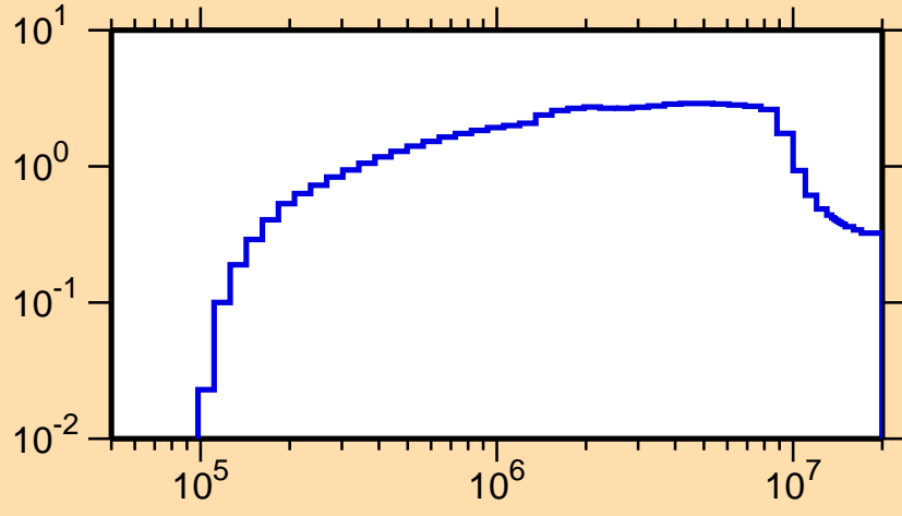
\sigma vs. E for ^{182}\text{W}(n,\text{inel.})
