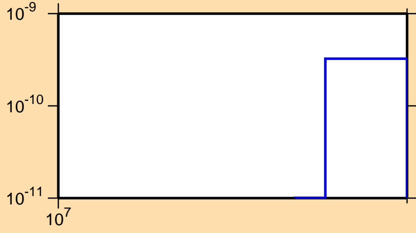
\sigma vs. E for ^{182}\text{W}(n,\text{He}3)
