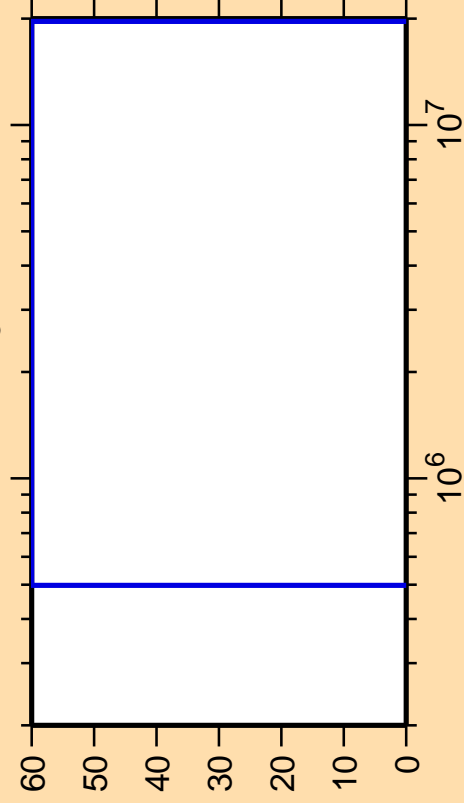
\Delta\sigma/\sigma vs. E for ^{182}\text{W}(n,n_3)
