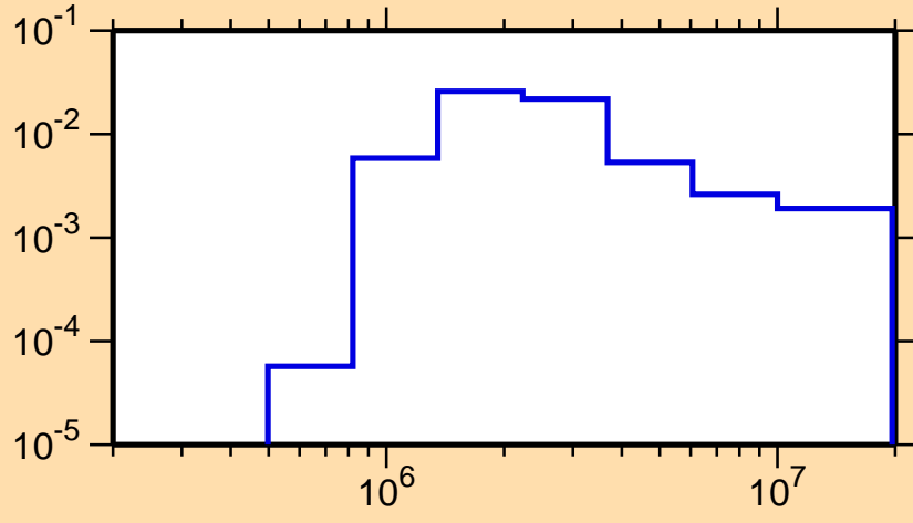
\sigma vs. E for ^{182}\text{W}(n,n_3)
