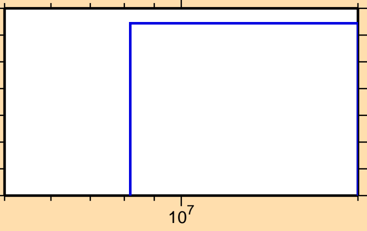
\sigma vs. E for ^{182}\text{W}(n,p\alpha)
