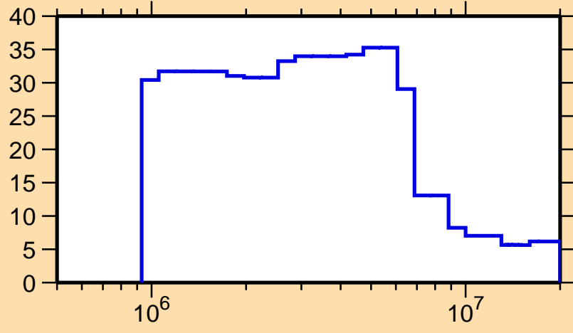
\Delta\sigma/\sigma vs. E for ^{183}\text{W}(n, tot.)
