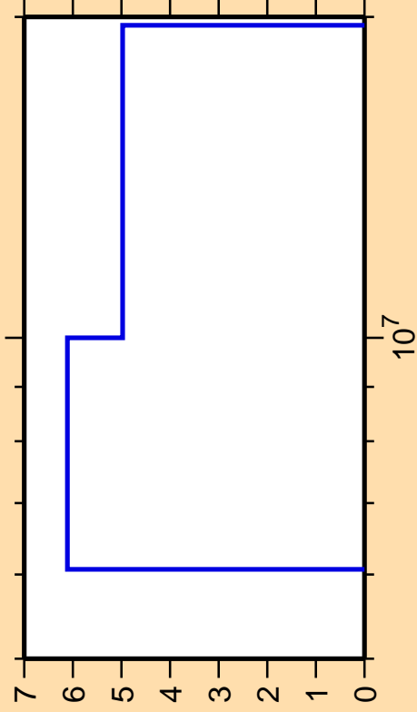
\Delta\sigma/\sigma vs. E for ^{183}\text{W}(n,2n)
