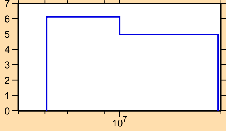
\Delta\sigma/\sigma vs. E for ^{183}\text{W}(n,2n)
