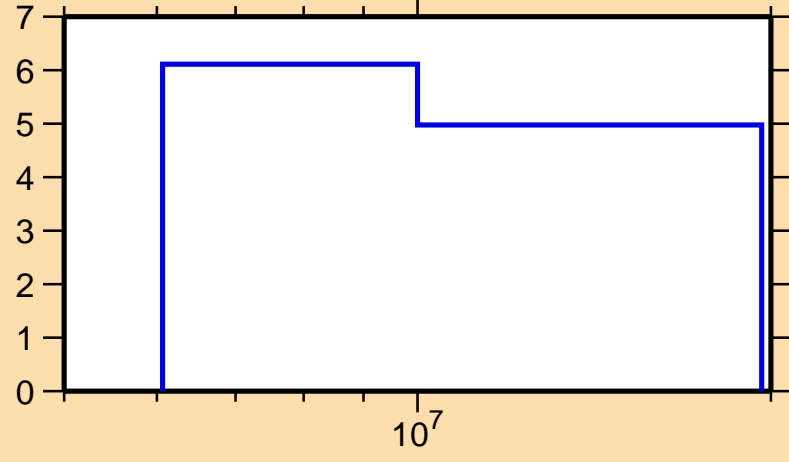
\Delta\sigma/\sigma vs. E for ^{183}\text{W}(n,2n)
