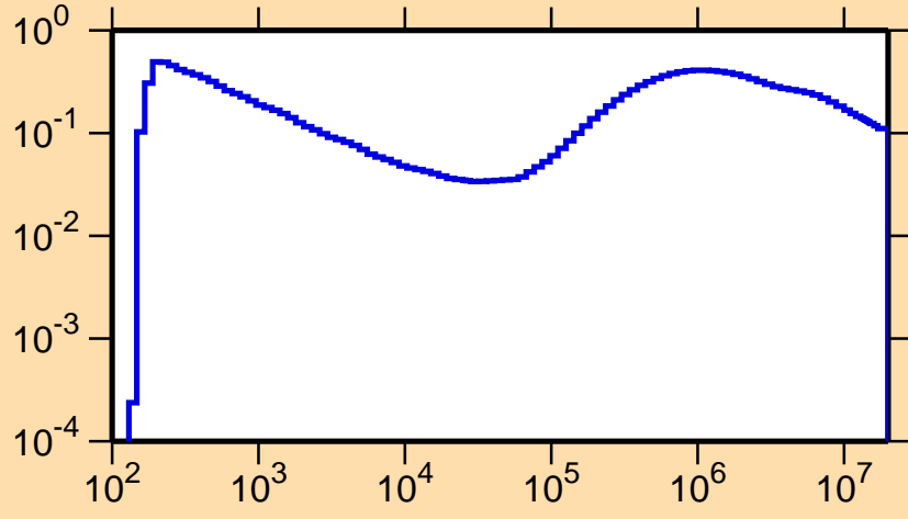
\sigma vs. E for ^{183}\text{W}(n,n_2)
