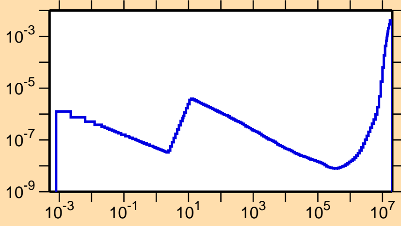
\sigma vs. E for ^{183}\text{W}(n,\alpha)
