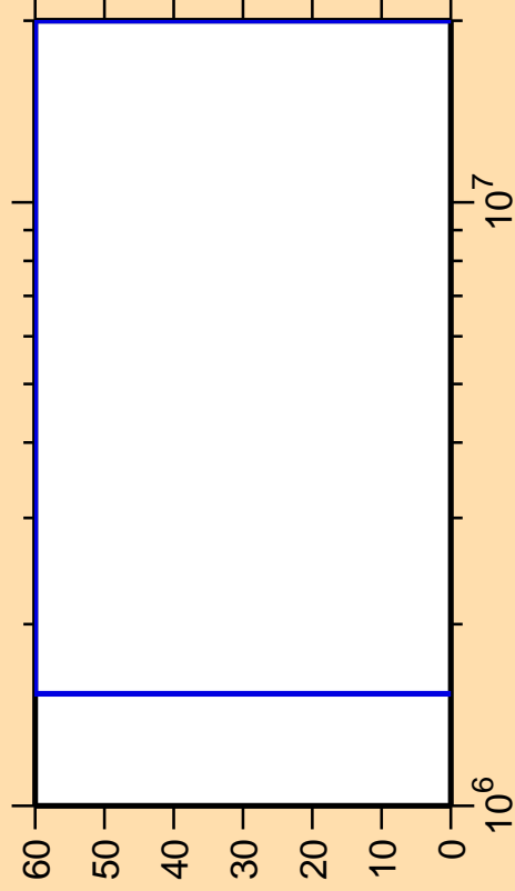
\Delta\sigma/\sigma vs. E for ^{184}\text{W}(n,\text{ncont.})
