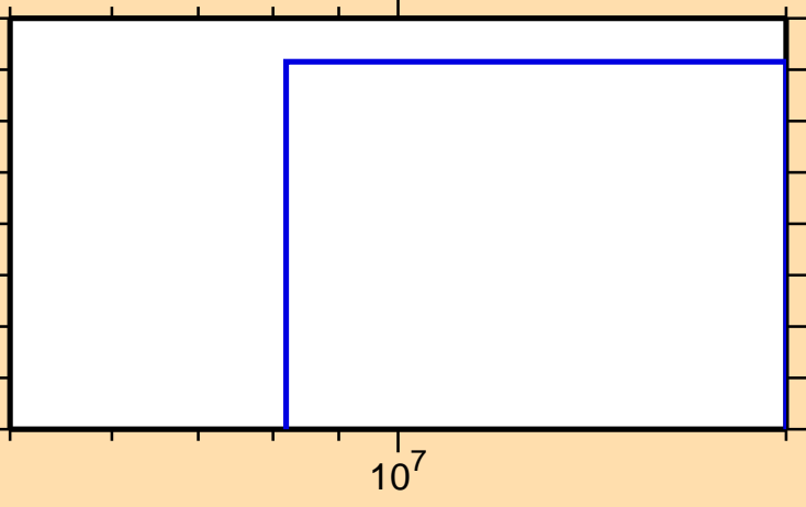
\sigma vs. E for ^{184}\text{W}(n,3n)
