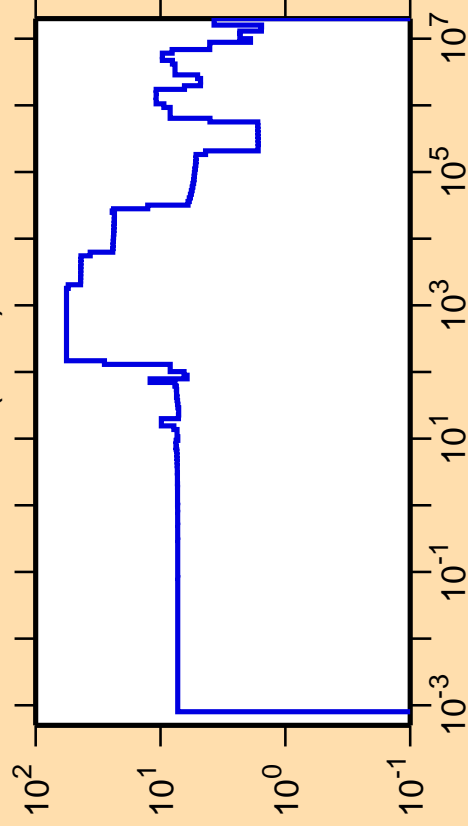
\Delta\sigma/\sigma vs. E for ^{185}\text{W}(n,\text{el.})
