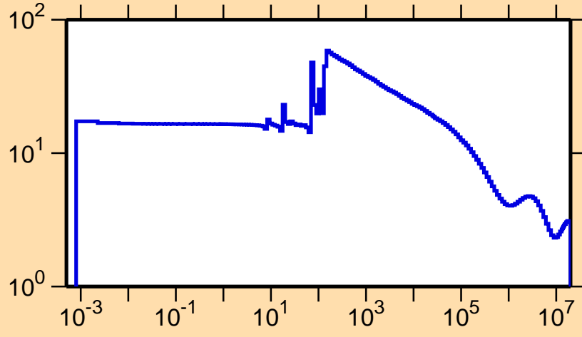
\sigma vs. E for ^{185}\text{W}(n,\text{el.})
