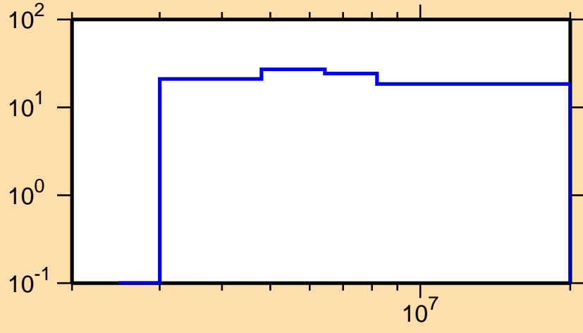
\Delta\sigma/\sigma vs. E for ^{185}\text{W}(n,p)
