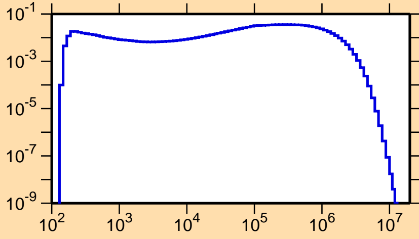
\sigma vs. E for ^{185}\text{W}(n,n_3)
