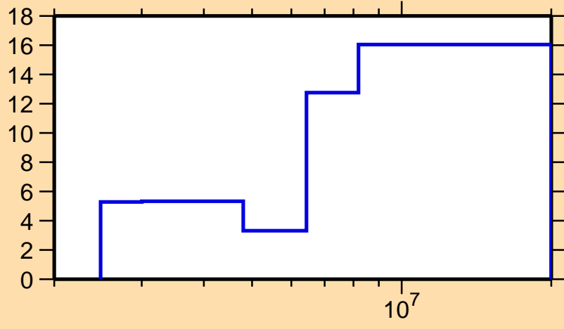
\Delta\sigma/\sigma vs. E for ^{185}\text{W}(n,ncont.)
