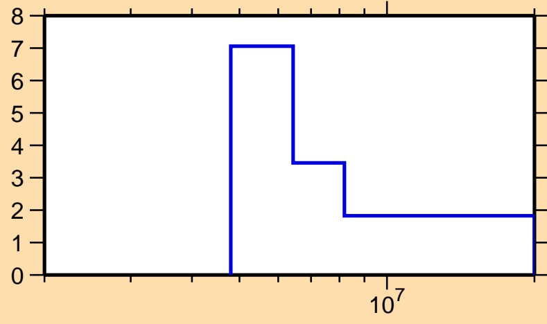
\Delta\sigma/\sigma vs. E for ^{185}\text{W}(n,\text{el.})
