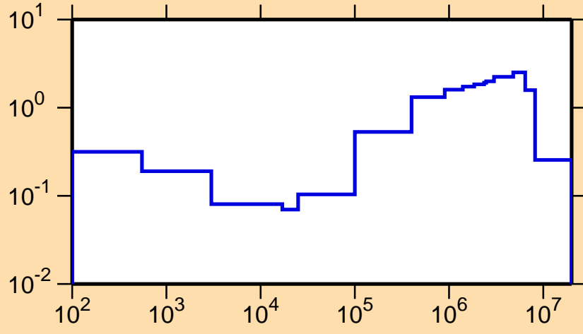
\sigma vs. E for ^{185}\text{W}(n,\text{inel.})
