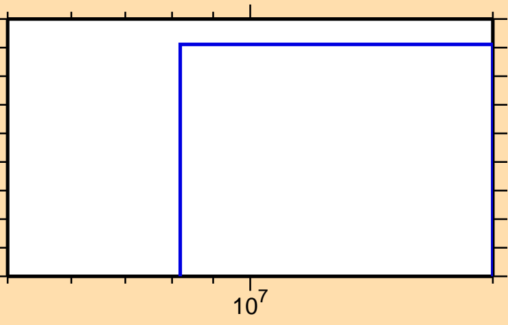
\sigma vs. E for ^{185}\text{W}(n,2n\alpha)
