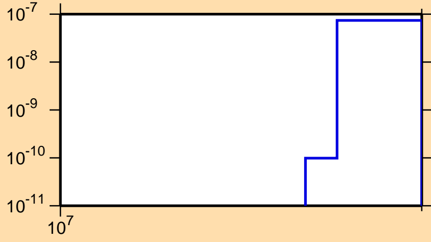
\sigma vs. E for ^{186}\text{W}(n,nt)
