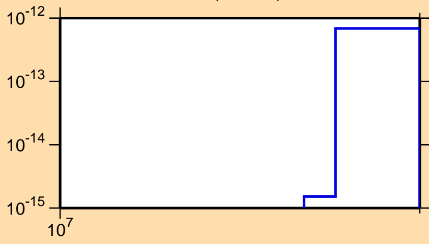
\sigma vs. E for ^{186}\text{W}(n,\text{He3})
