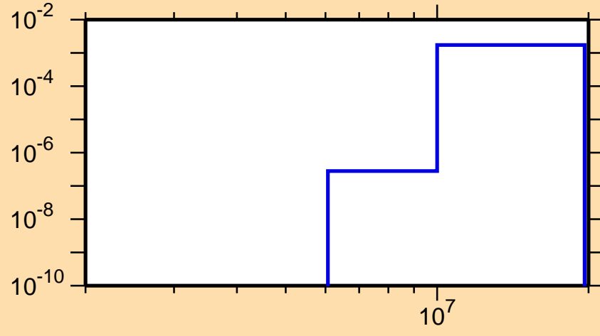
\sigma vs. E for ^{186}\text{W}(n,p)
