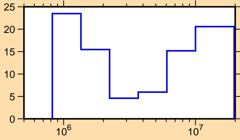
\Delta\sigma/\sigma vs. E for ^{187}\text{W}(n,ncont.)
