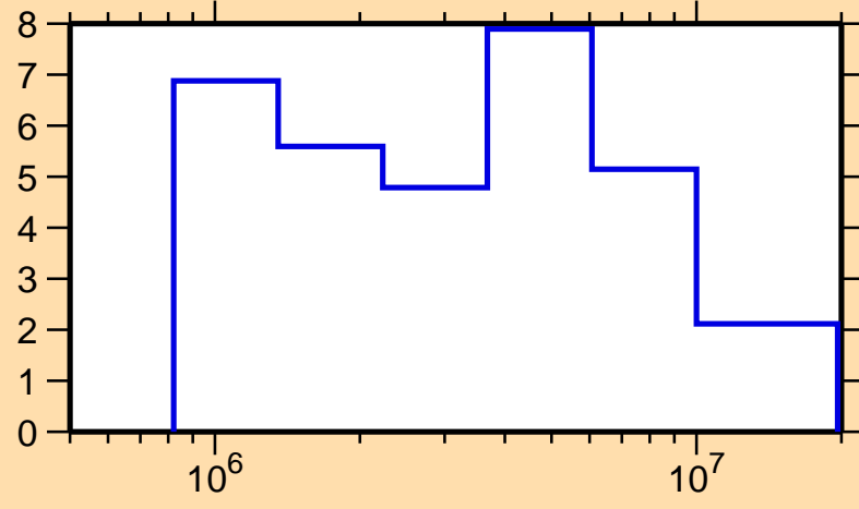
\Delta\sigma/\sigma vs. E for ^{187}\text{W}(n, \text{el.})
