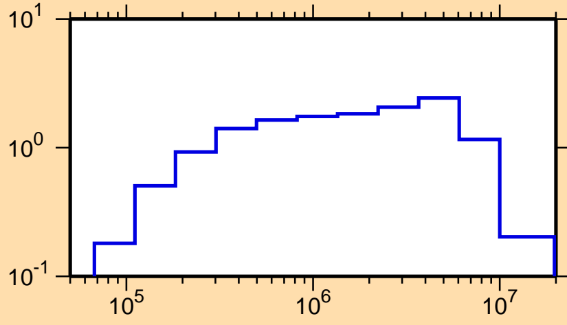
\sigma vs. E for ^{187}\text{W}(n,\text{inel.})
