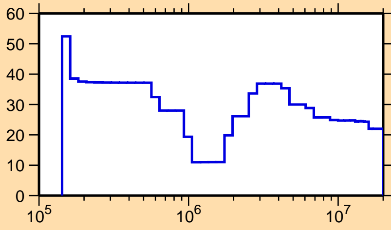
\Delta\sigma/\sigma vs. E for ^{188}\text{W}(n,n_1)
