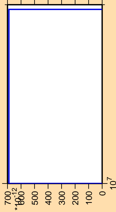
\Delta\sigma/\sigma vs. E for ^{188}\text{W} (mt 11)
