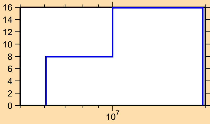
\Delta\sigma/\sigma vs. E for ^{188}\text{W}(n,ncont.)
