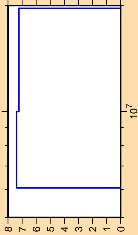
\Delta\sigma/\sigma vs. E for ^{188}\text{W}(n,2n)
