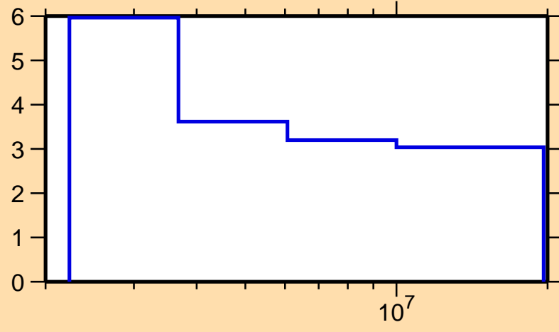
\Delta\sigma/\sigma vs. E for ^{188}\text{W}(n,\text{nonel.})
