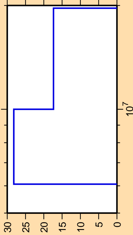
\Delta\sigma/\sigma vs. E for ^{188}\text{W}(n,p)
