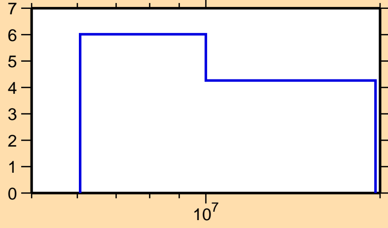
\Delta\sigma/\sigma vs. E for ^{188}\text{W}(n,el.)
