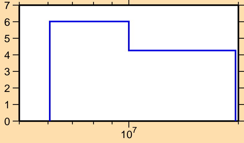
\Delta\sigma/\sigma vs. E for ^{188}\text{W}(n,\text{el.})
