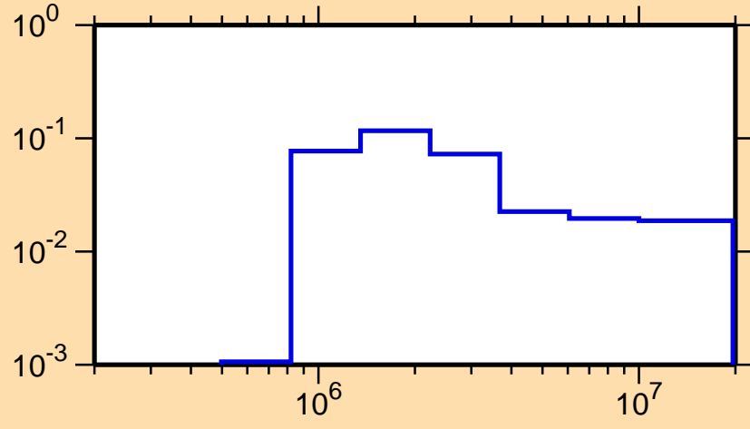
\sigma vs. E for ^{188}\text{W}(n,n_4)
