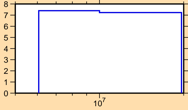
\Delta\sigma/\sigma vs. E for ^{188}\text{W}(n,2n)
