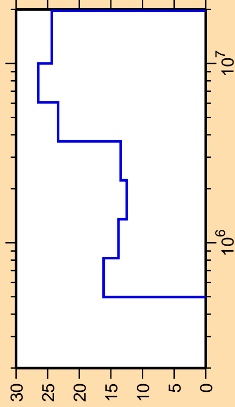
\Delta\sigma/\sigma vs. E for ^{188}\text{W}(n,n_4)
