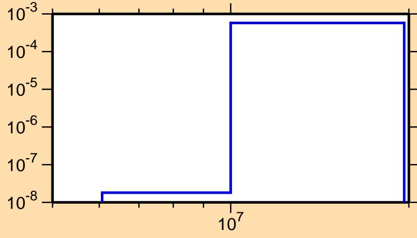
\sigma vs. E for ^{188}\text{W}(n,p)
