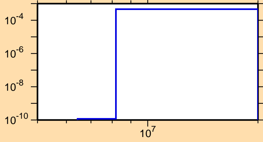
\sigma vs. E for ^{188}\text{W}(n,p)
