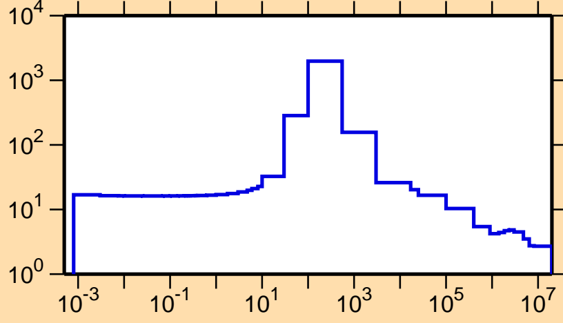
\sigma vs. E for ^{188}\text{W}(n,\text{el.})
