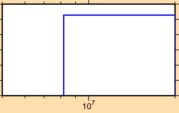
\sigma vs. E for ^{188}\text{W}(n,d)
