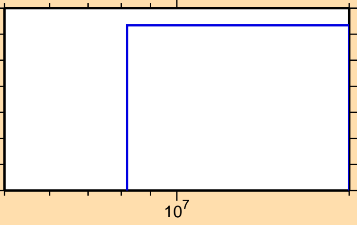
\sigma vs. E for ^{188}\text{W}(n,3n)
