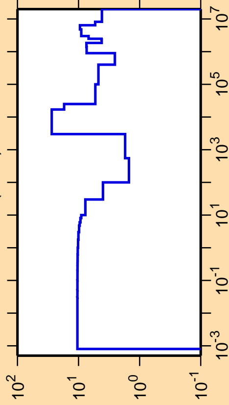
\Delta\sigma/\sigma vs. E for ^{188}\text{W}(n,\text{el.})
