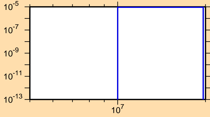
\sigma vs. E for ^{189}\text{W}(n,np)
