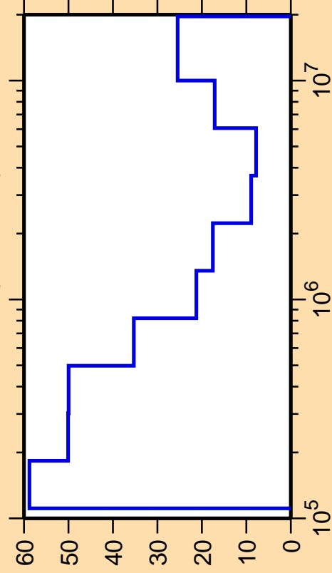
\Delta\sigma/\sigma vs. E for ^{189}\text{W}(n,\text{ncont.})
