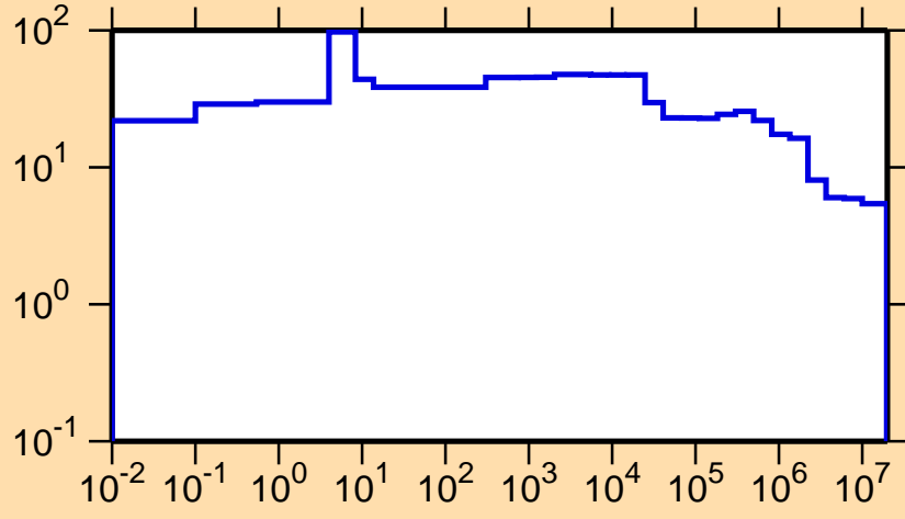
\Delta\sigma/\sigma vs. E for ^{189}\text{W}(n,\text{nonel.})
