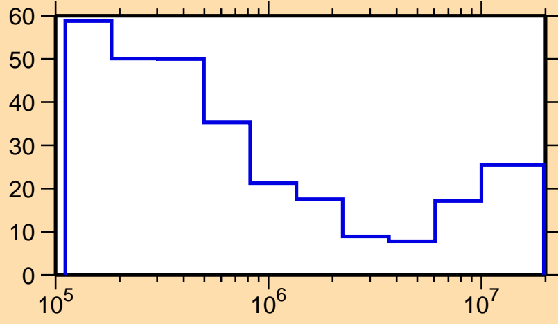
\Delta\sigma/\sigma vs. E for ^{189}\text{W}(n,n\text{cont.})
