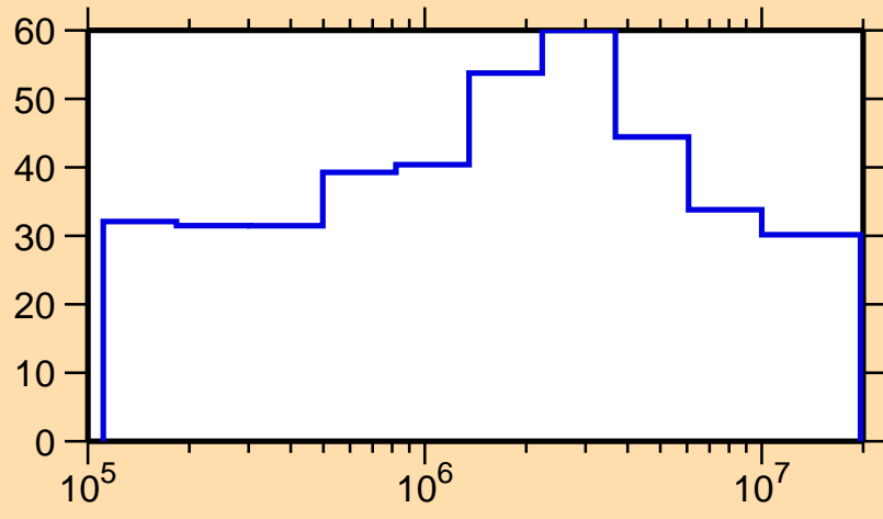
\Delta\sigma/\sigma vs. E for ^{189}\text{W}(n,n_1)
