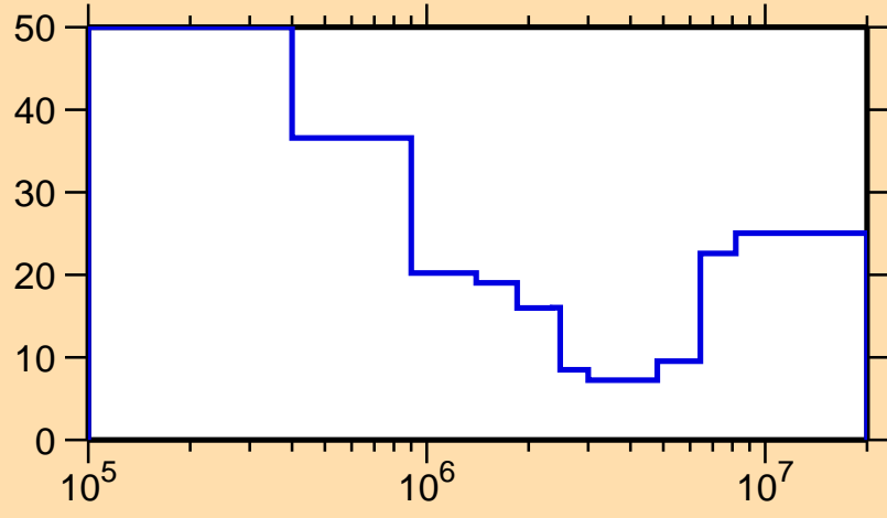
\Delta\sigma/\sigma vs. E for ^{189}\text{W}(n,n\text{cont.})
