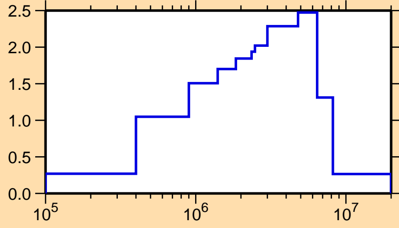
\sigma vs. E for ^{189}\text{W}(n,\text{inel.})
