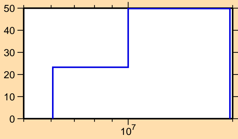
\Delta\sigma/\sigma vs. E for ^{190}\text{W}(n,ncont.)
