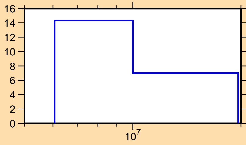
\Delta\sigma/\sigma vs. E for ^{190}\text{W}(n,el.)
