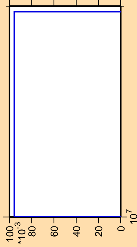
\Delta\sigma/\sigma vs. E for ^{190}\text{W}(n,2np)
