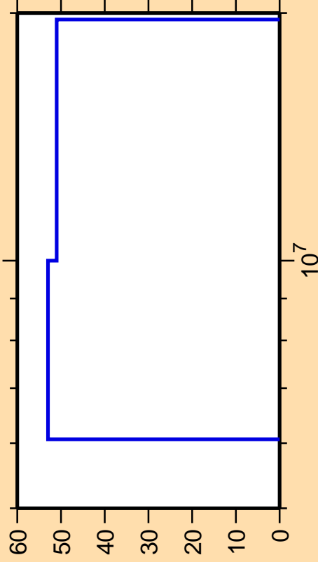
\Delta\sigma/\sigma vs. E for ^{190}\text{W}(n,p)
