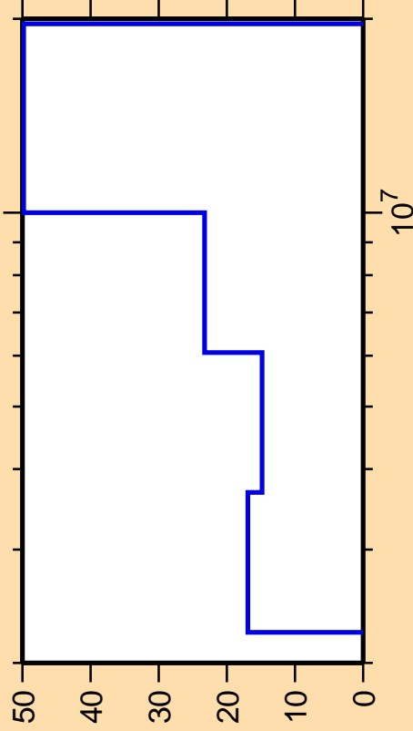
\Delta\sigma/\sigma vs. E for ^{190}\text{W}(n,n\text{cont.})
