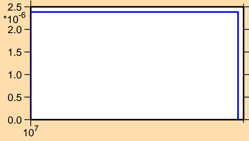
\sigma vs. E for ^{190}\text{W}(n,t)
