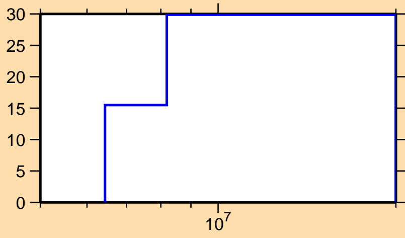
\Delta\sigma/\sigma vs. E for ^{190}\text{W}(n,2n)
