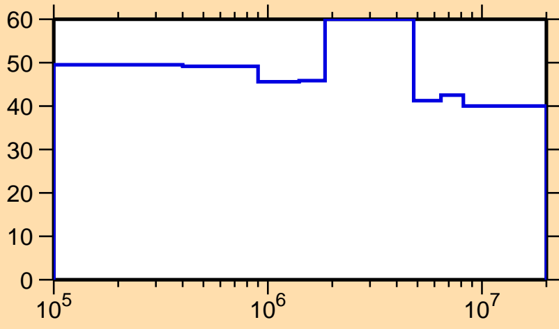
\Delta\sigma/\sigma vs. E for ^{190}\text{W}(n,n_1)
