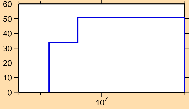
\Delta\sigma/\sigma vs. E for ^{190}\text{W}(n,ncont.)
