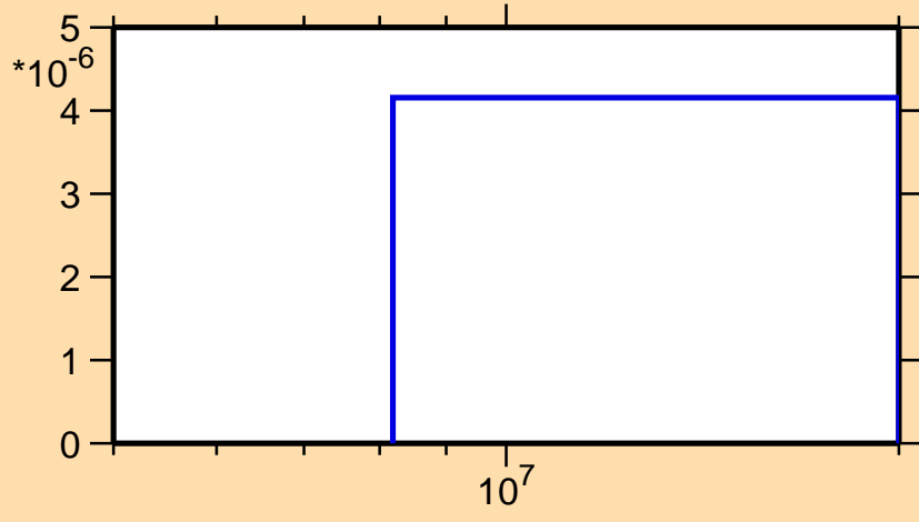
\sigma vs. E for ^{190}\text{W}(n,d)
