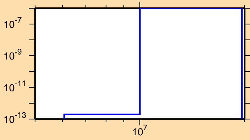
\sigma vs. E for ^{191}\text{W}(n,n\alpha)
