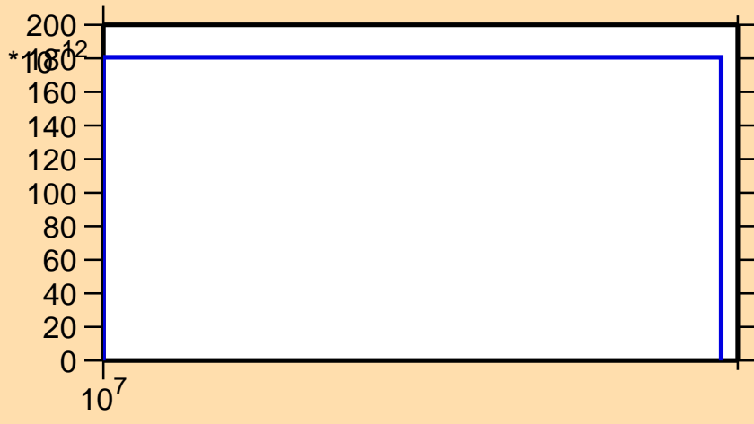
\sigma vs. E for ^{191}\text{W}(n,2n\alpha)
