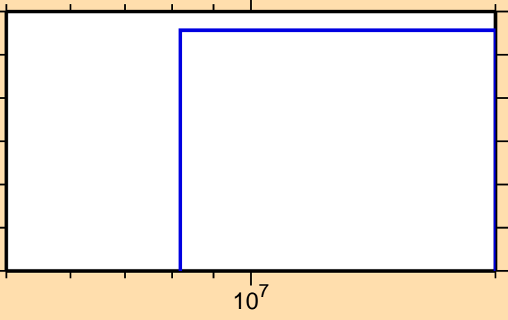
\sigma vs. E for ^{191}\text{W}(n,d)
