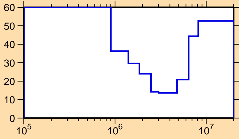
\Delta\sigma/\sigma vs. E for ^{191}\text{W}(n,n\text{cont.})
