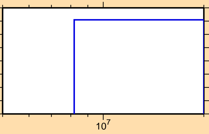
\sigma vs. E for ^{191}\text{W}(n,2np)
