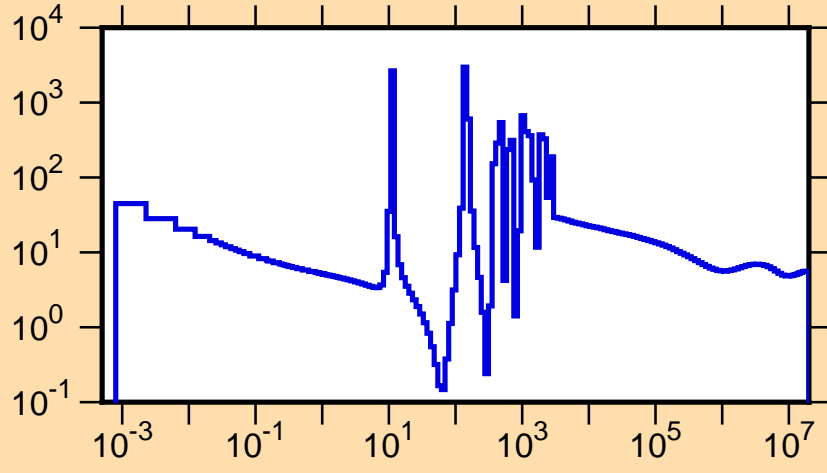
\sigma vs. E for ^{192}\text{W}(n,\text{tot.})
