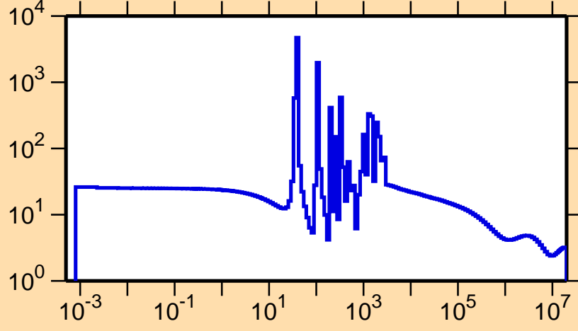
\sigma vs. E for ^{193}\text{W}(n,\text{el.})
