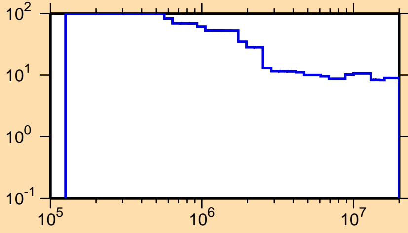
\Delta\sigma/\sigma vs. E for ^{193}\text{W}(n, nonel.)
