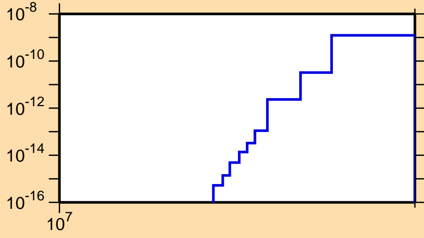
\sigma vs. E for ^{193}\text{W}(n,2n\alpha)
