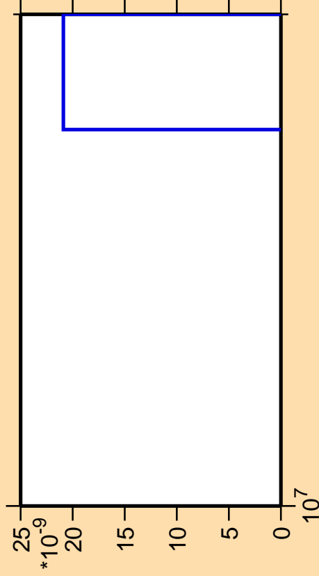
\Delta\sigma/\sigma vs. E for ^{193}\text{W} (mt 11)
