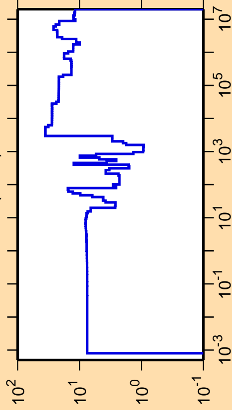
\Delta\sigma/\sigma vs. E for ^{193}\text{W}(n,\text{el.})
