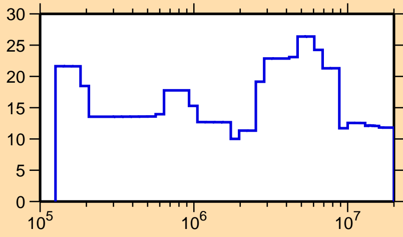
\Delta\sigma/\sigma vs. E for ^{193}\text{W}(n, el.)
