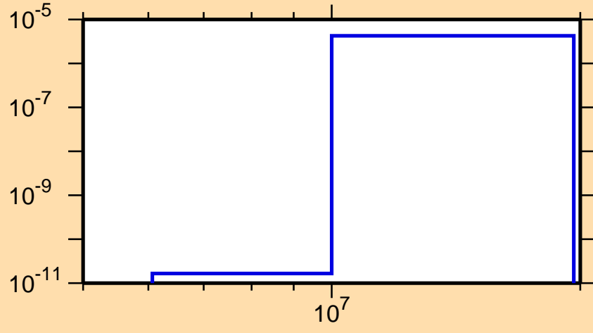
\sigma vs. E for ^{193}\text{W}(n,\alpha)
