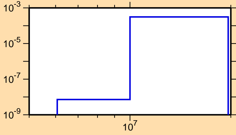
\sigma vs. E for ^{193}\text{W}(n,p)
