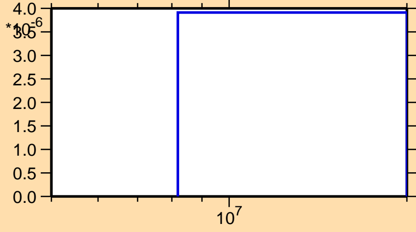
\sigma vs. E for ^{193}\text{W}(n,d)
