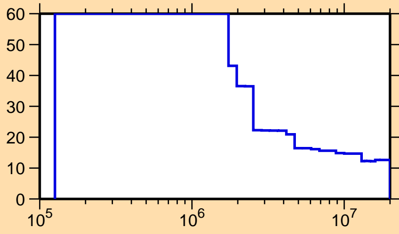
\Delta\sigma/\sigma vs. E for ^{194}\text{W}(n, nonel.)
