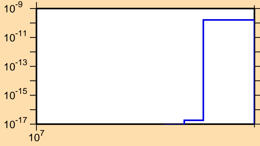
\sigma vs. E for ^{194}\text{W}(n,\text{nd})
